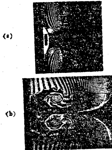
Figure 6. Hydrogen Bubble Time Line Display of the Startup Eddies Behind a Two-dimensional Plate
