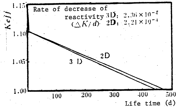
Figure 4. Rate of Decrease of the Reactivity in 3-D and 2-D Calculations
