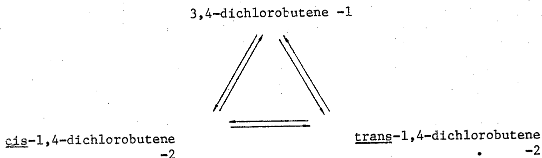
Figure 1. Isomerization of Dichlorobutene
