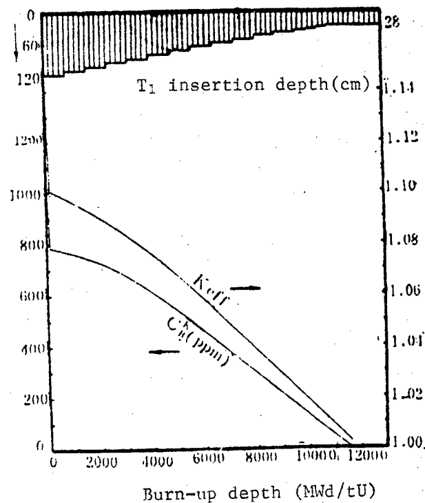
Figure 2. Variation of the Effective Breeding Coefficient K_{eff} and the Critical Boron Concentration C_B^k as a function of burn-up
