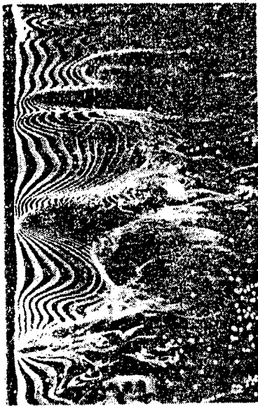
Figure 3. Display of an Even Flow Field's Hydrogen Bubble Time Line
