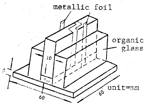
Figure 2. Diagram of Organic Glass Test Set
