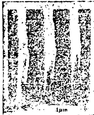
Figure 2. The pattern made by X-ray lithography on a PMMA film features a length/width ratio of 10.
