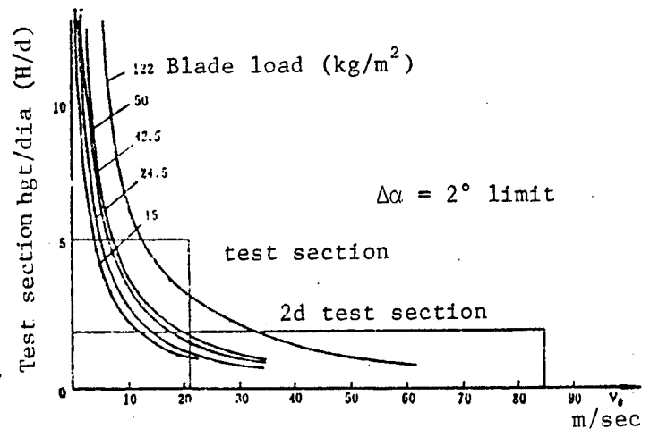
Figure 5. Simulation Ability for Blade Load
