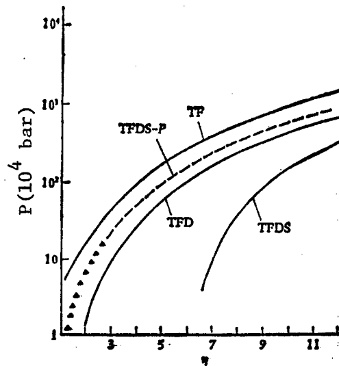
Figure 3. Relationship Between Pressure P and Compression Ratio \eta for K
