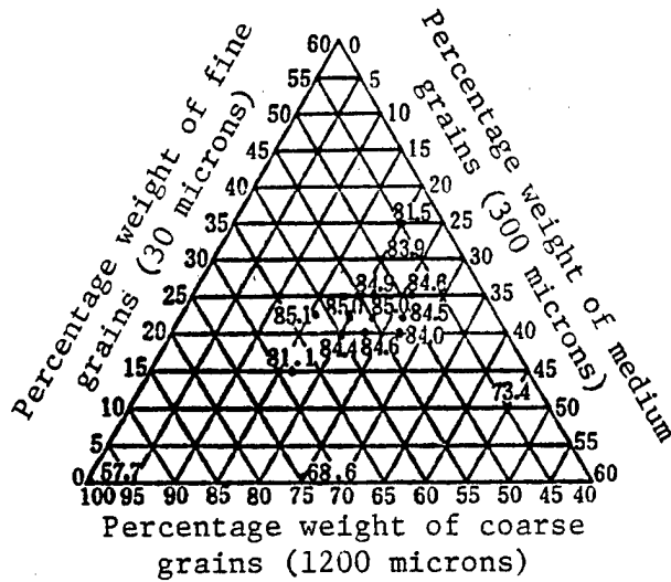
Fig. 1. Proportional relationship of coarse, medium, and fine granularity and effective density of "once method" (U·Pu) 2 O 2 microspheres (fast reactor casing)
