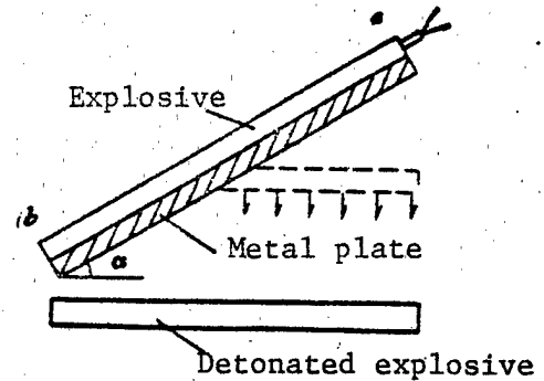
Figure 5. C Type Linear Wave
