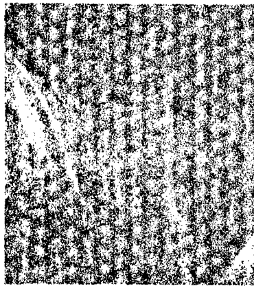
Figure 5. Photorecord of a "normal" detonation. The photograph was taken by a camera with increased resolving power. A mixture of 2\text{H}_2 + \text{O}_2 , p_0 = 760\text{mm} of mercury; d = 15\text{ mm} ; increased in comparison with the characteristic along the z -axis: G = 3 ; time scale t on the axis: 1 mm equals 0.2 microseconds.
