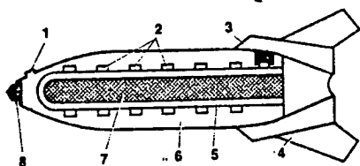
Figure 1. Binary aerial bomb with the toxic agent VX: 1 -- fill hole; 2 -- mixer; 3 -- motor; 4 -- tail fins; 5 -- steel tube; 6 -- liquid component; 7 -- powder (sulfur); 8 -- fuze.
