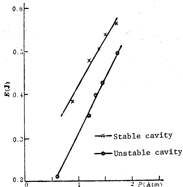
Figure 5. Laser Output Energy vs Rail Gap Switch Gas Pressure for Stable and Unstable Cavities
