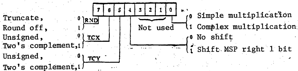
Figure 3. Instruction Format of Fast ALU
