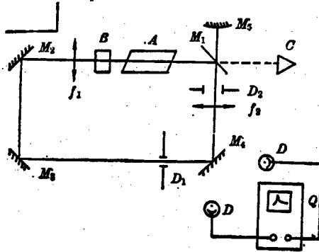
Figure 1. Experimental set-up
