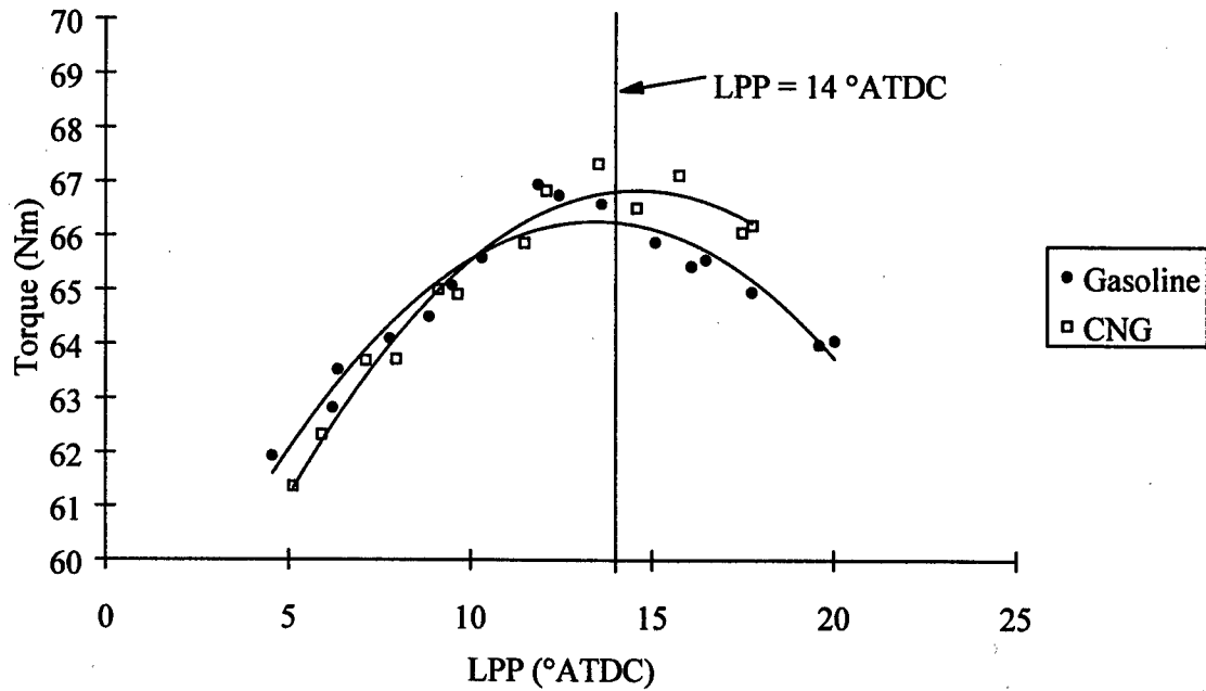
Figure 6. Basis for Ignition Timing Control Using In-Cylinder Pressure
