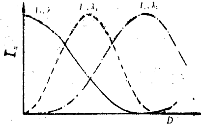
Figure 1. Theoretical Curve of Normalized Output Light Intensity I_n Following Changes in Density D
