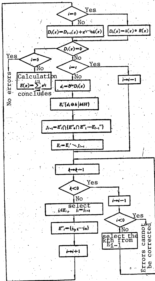
Figure 1. Block Diagram of the Cyclic Decoding Program
