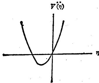
Figure 2. Potential V(\eta) When \omega_0 = k_0 \mathcal{V}_z
