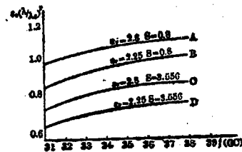
Figure 4. Dispersion characteristics of the domestic substrate (measured)
