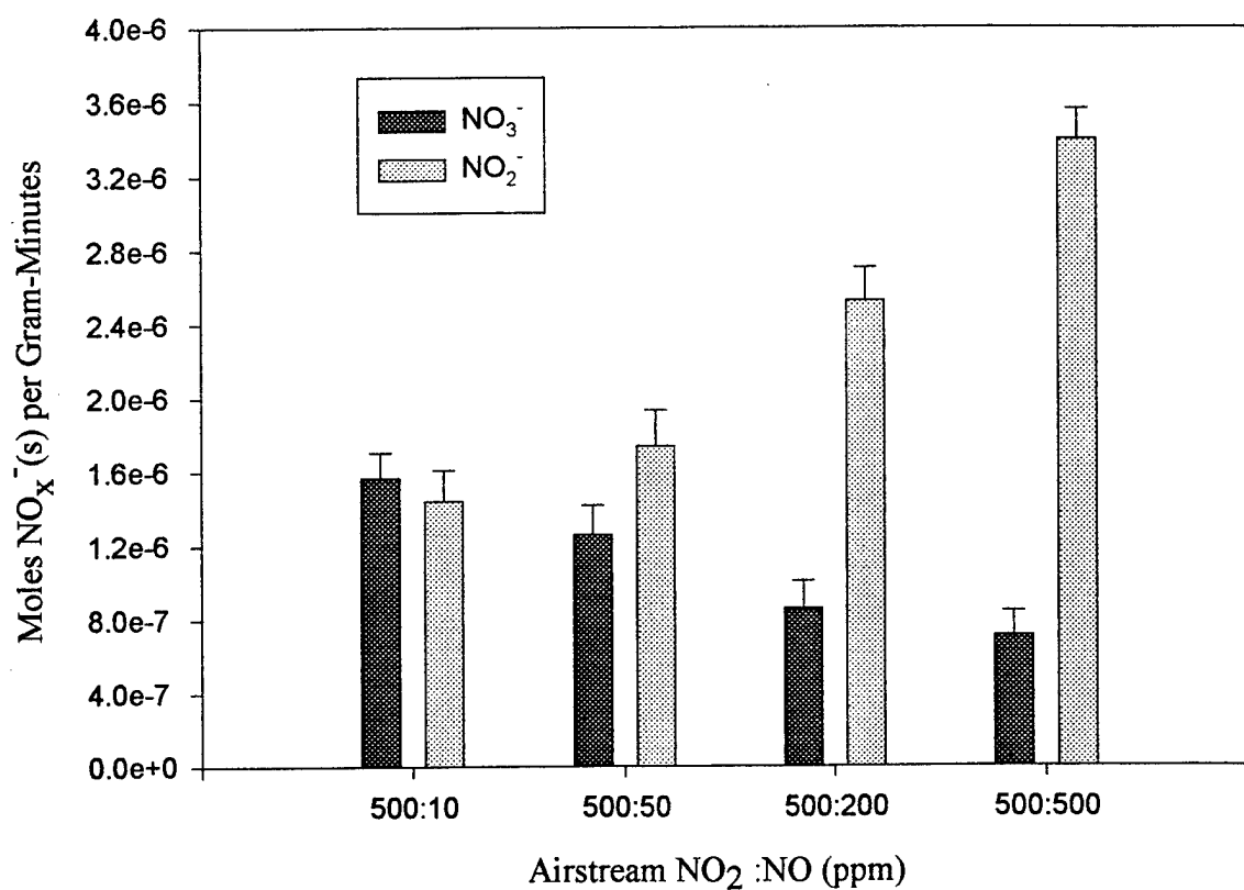
Figure 3-25. Nitrate and Nitrite Moles per Gram Alumina per Minute Exposure Time for \text{K}_2\text{CO}_3 -Treated Alumina Exposed to Varying \text{NO} Concentrations in Airstream, 200C
