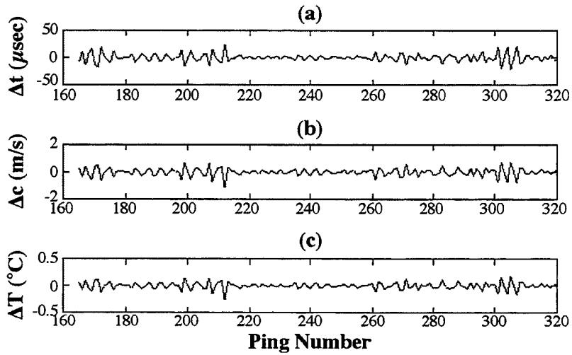
Figure 20: Flight time, sound speed and temperature fluctuations for run 10.1-A.
