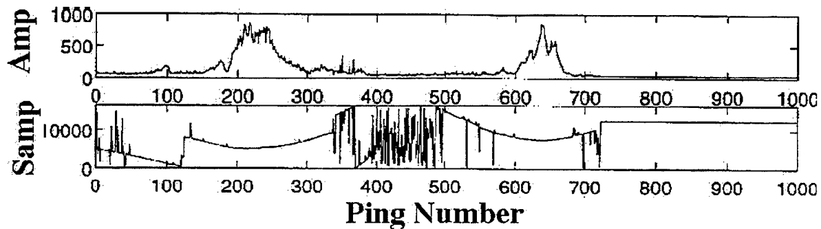
Figure 3: A summary of the acoustic data for run 11, channel 1. Plotted are maximum acoustic amplitude (top) and arrival time sample (bottom) vs. ping number for the entire run.
