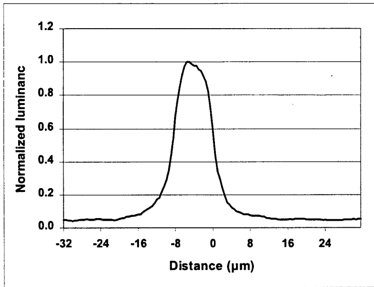
Figure 23. Normalized Kaiser 12- \mu\text{m} horizontal linespread curve.
