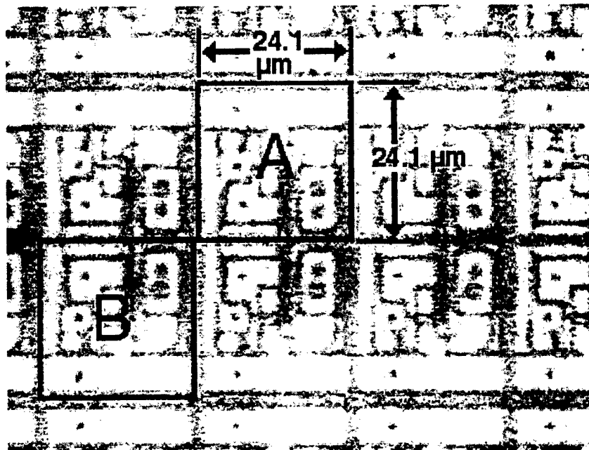
Figure 6. Enlarged subsection with light enhancement. Two pixels are highlighted (pixels A and B). Using computer mensuration, we measured pixel pitch to be 24.1 μm, which also equates to the pixel size.
