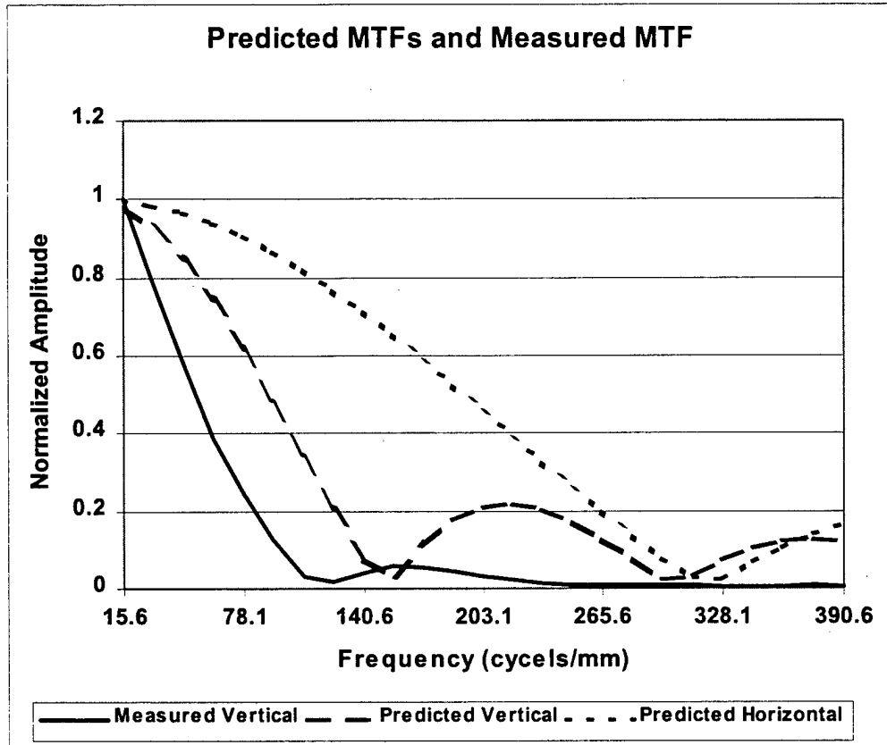
Figure 27. Horizontal and vertical predicted MTFs compared with the measured MTF. The predicted vertical MTF was based upon a fill factor of 0.55 whereas the predicted horizontal MTF was based upon a fill factor of 0.26.
