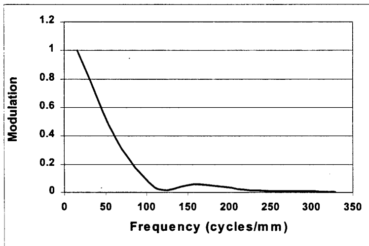
Figure 24. Normalized vertical MTF for the Kaiser 12- \mu\text{m} display.
