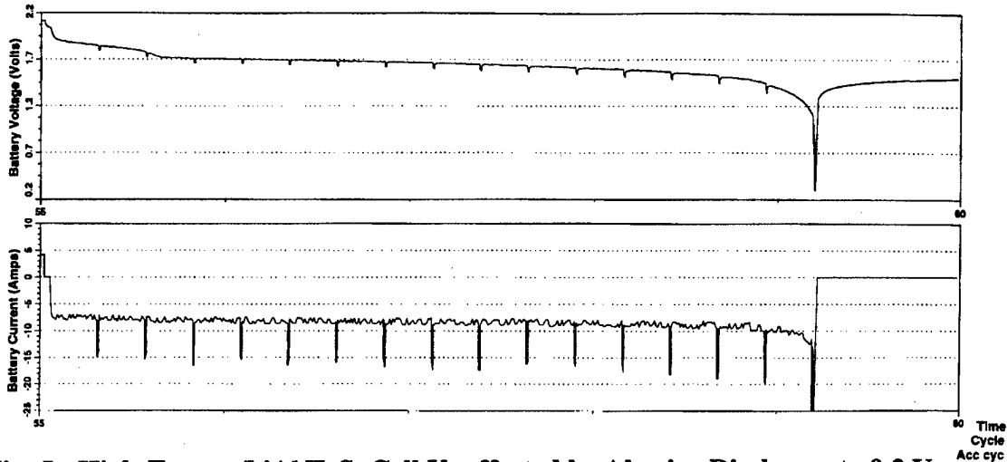
Fig. 5: High-Energy LiAl/FeS 2 Cell Unaffected by Abusive Discharge to 0.2 V
