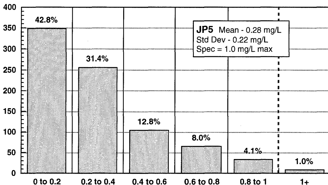
Chart 14 Distribution of Particulate Contamination by Volume Received for 1997 (Millions of Gallons)
