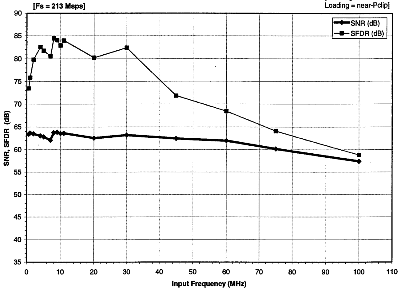
Figure 3. ADC Baseband Performance: SNR and SFDR versus Fin for Single-Ended Analog Input (no input transformer).
