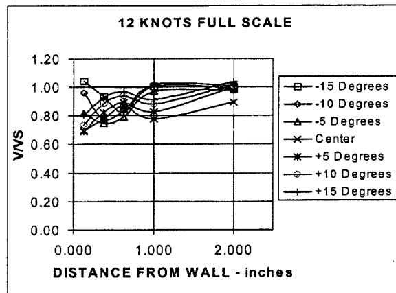
FIG. 12 Self-Propelled Capture Area Velocities
