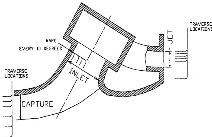
FIG. 4 Measurement Stations
