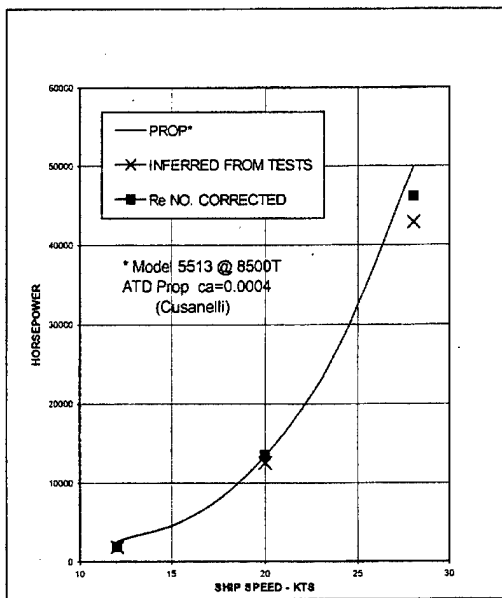
FIG. 2 VMP/PROPELLER COMPARISONS
