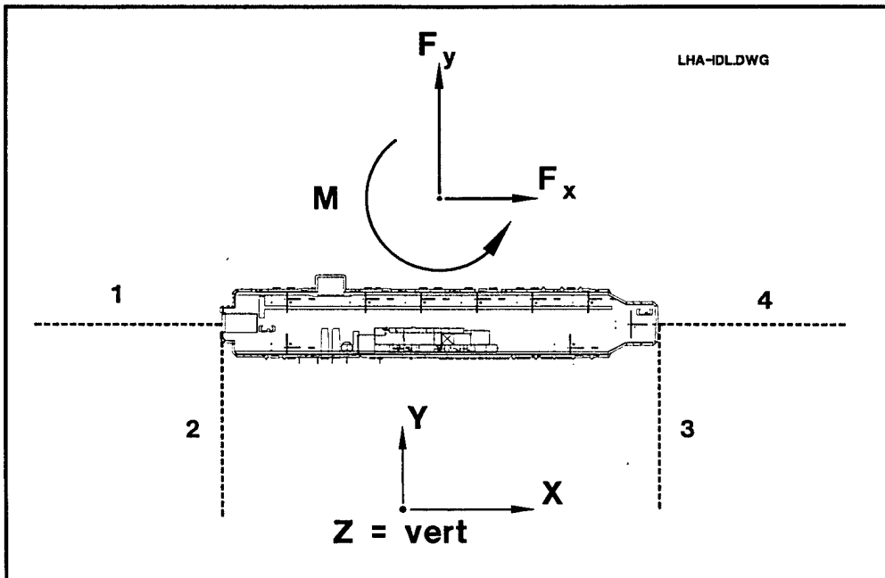
Figure 3.8 The Optimum Ideal Mooring (Lines Parallel to the Water Surface and Breasting Lines Spaced at X=0.5 * L from Midships)
