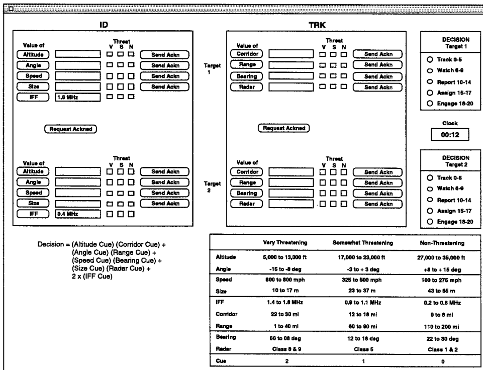
Fig. 2 — The subject's screen for computer acknowledgment modes CACR and CAVR
