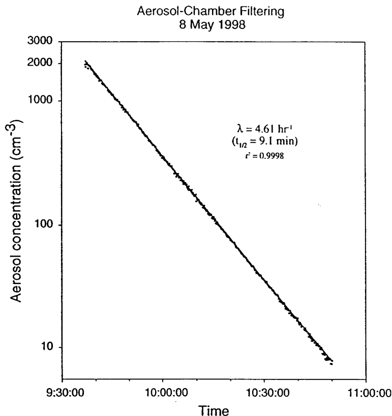
Fig. 1 – Filtering efficiency for total aerosol concentration
