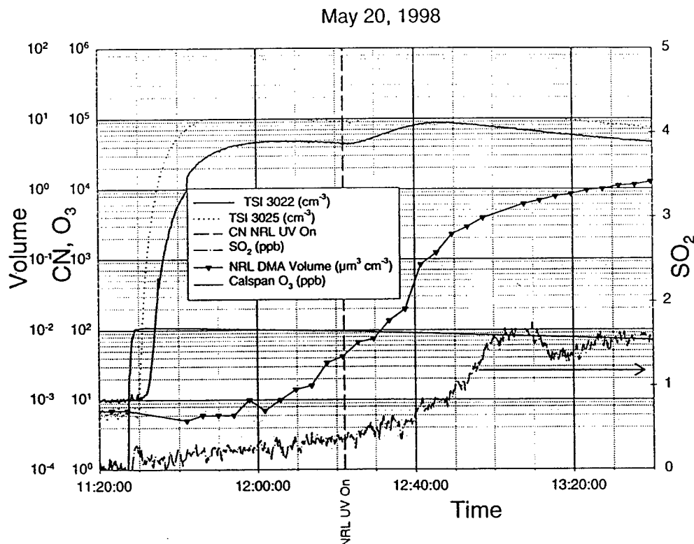
Fig. 31 – Aerosol formation during photolysis of DMS in concentration of about 30 ppb
