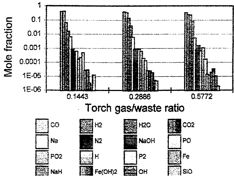
Figure 5.8 Destruction of NSW with a plasma torch under oxidizing conditions gives these predicted gaseous products. This prediction is for oxygen as the torch gas, but air gives similar results except for a much greater amount of N 2 and more NO x .
