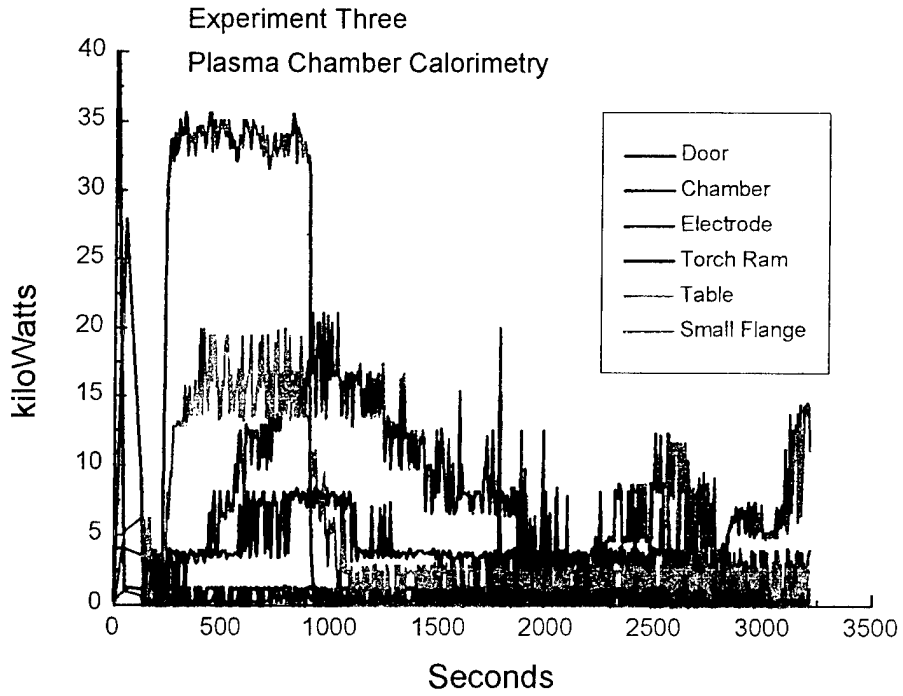
Figure B.14 - Experiment Three: Plasma Chamber Calorimetry
