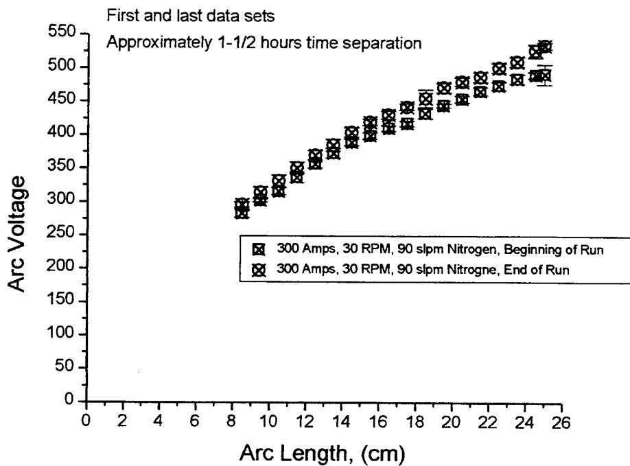
Figure 3.8 Arc Voltage Versus Arc Length Data: Experiment 5
