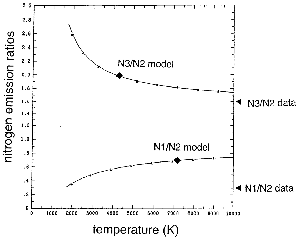
Figure 4.7 The solid lines are the calculated ratios for the N1/N2 and N3/N2 emission features of nitrogen assuming LTE conditions. The data from Figure 4.4 are marked on the right side. The model ratios arise from the CRE calculation described in the text.
