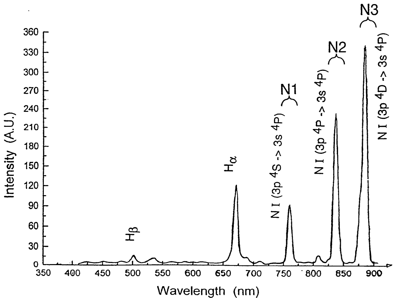
Figure 4.2 Sample optical spectrum of the plasma arc in the non-transferred mode taken at the center of the arc ( y = 0 ), 1 cm down from the torch nozzle. Each emission feature from neutral nitrogen (NI), denoted as N1, N2, and N3, is actually a complex of lines as described in the text. Two of the Balmer lines from hydrogen, H_{\alpha} and H_{\beta} , are also noted. The operating conditions are 333 Volts, 375 Amps, 125 kW, 100 slpm (standard liters per minute) of N_2 , with a H_2 seeding of 5 slpm.
