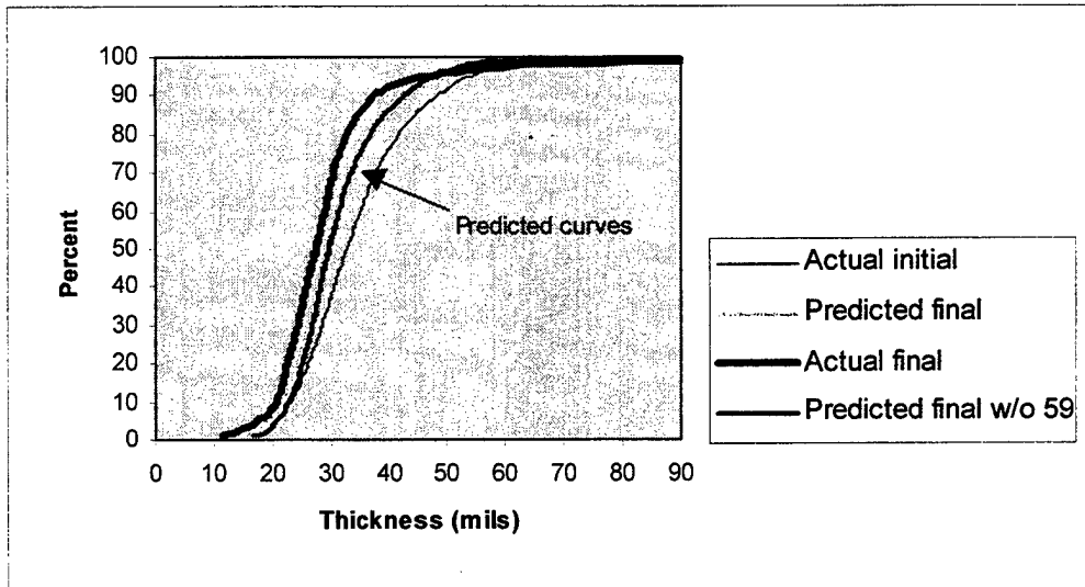
Figure 8. Model Comparison—Predictions for CVN 73(a) with and without data from CV 59.
