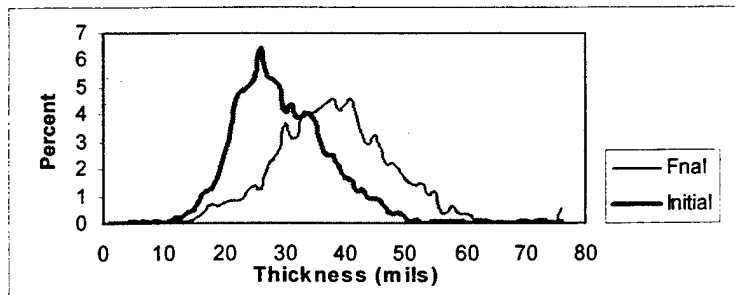
Figure 13. CVN 69 hull coating system thickness before and after two AF paint coats.
