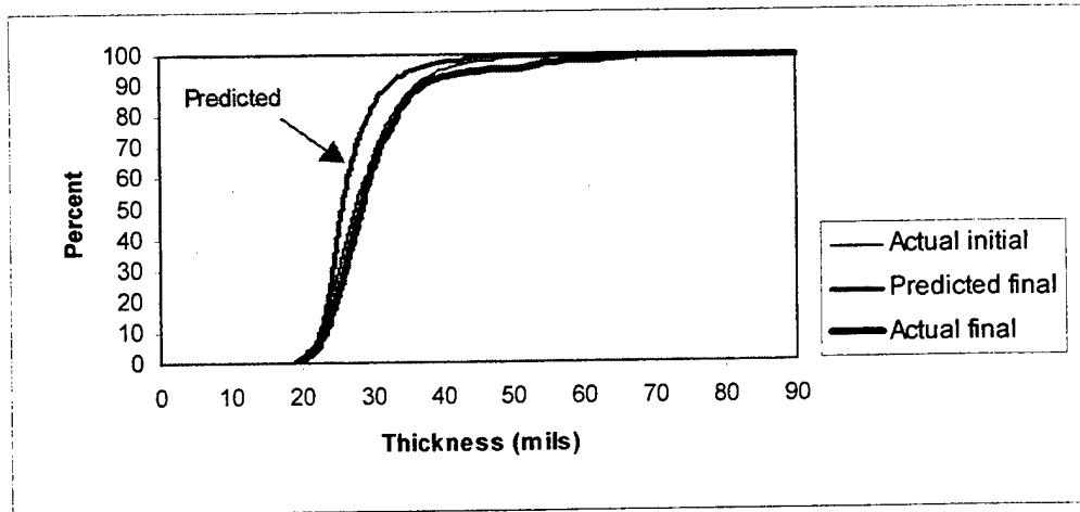
Figure 5. Model Validation—Predicting the coating system distribution of CVN 67.
