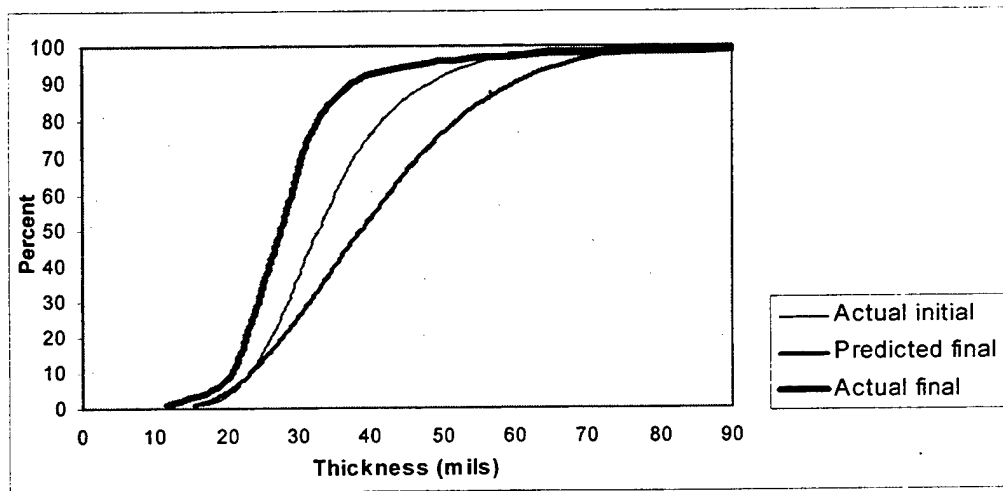
Figure 9. Model Validation—Predicting the coating system distribution of CVN 73(a).
