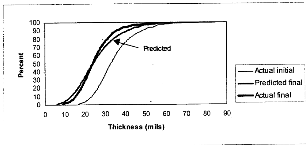
Figure 4. Model Validation—Predicting the coating system distribution of CVN 73(b).
