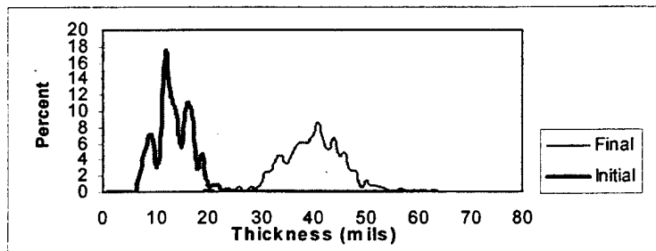
Figure 12. CVN 69 hull coating system thickness before and after four AF paint coats.
