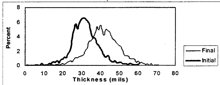
Figure 11. CV 64 hull coating system thickness before and after one AF paint coat.
