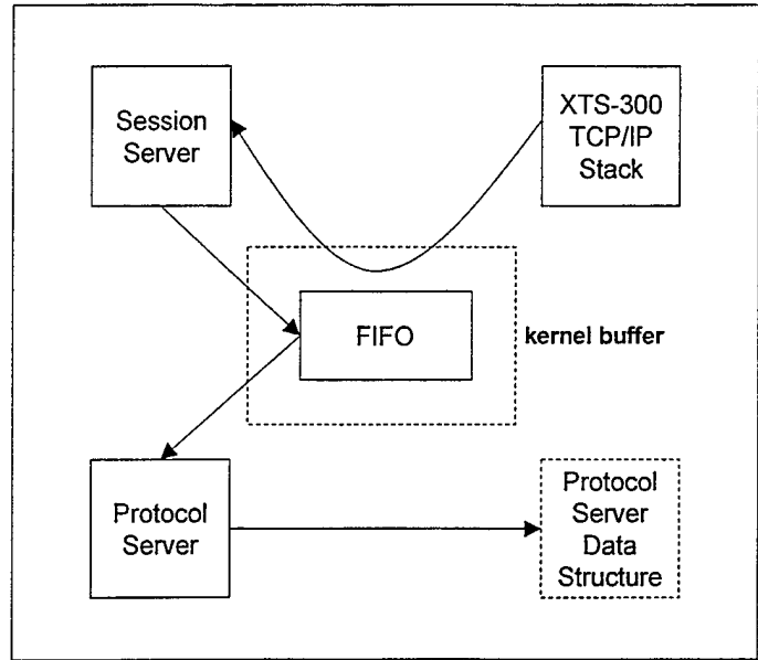
Figure 21. FIFO Data Flow
