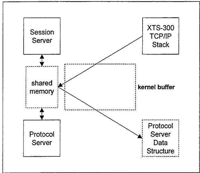
Figure 22. Shared Memory Data Flow [Ref. 22]
