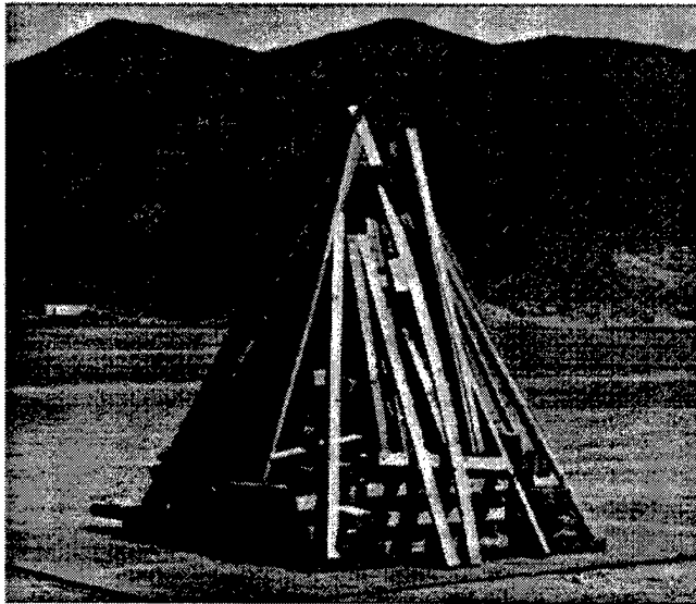
FIGURE 5. COMPLETED SETUP FOR TEST NO. 1
