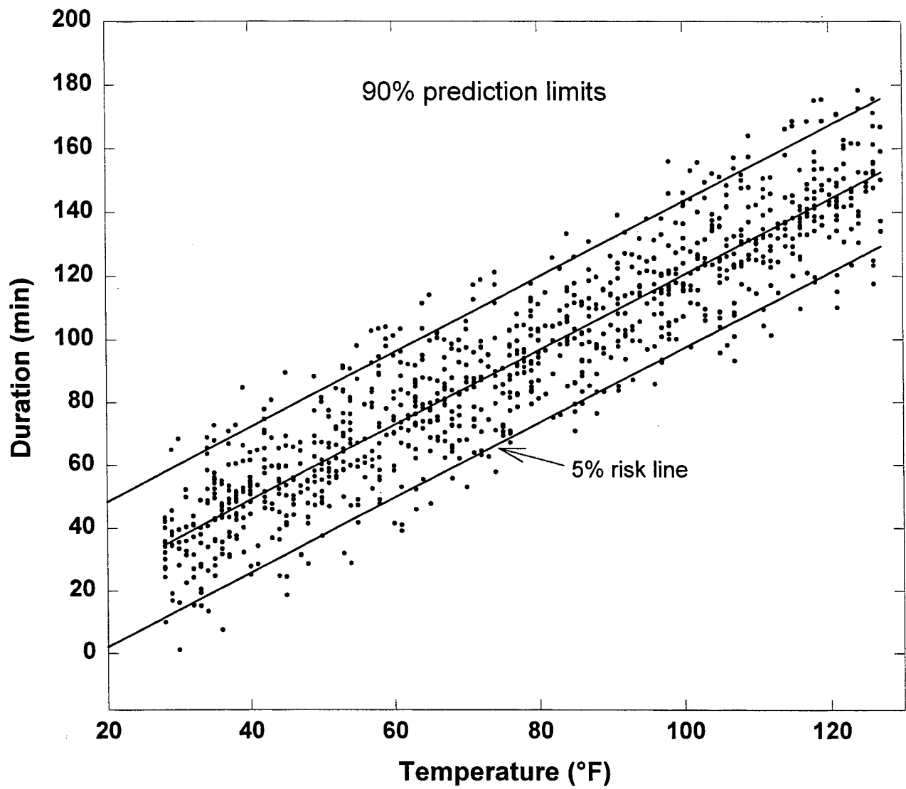
Figure 5. 90% prediction limits on the regression.
