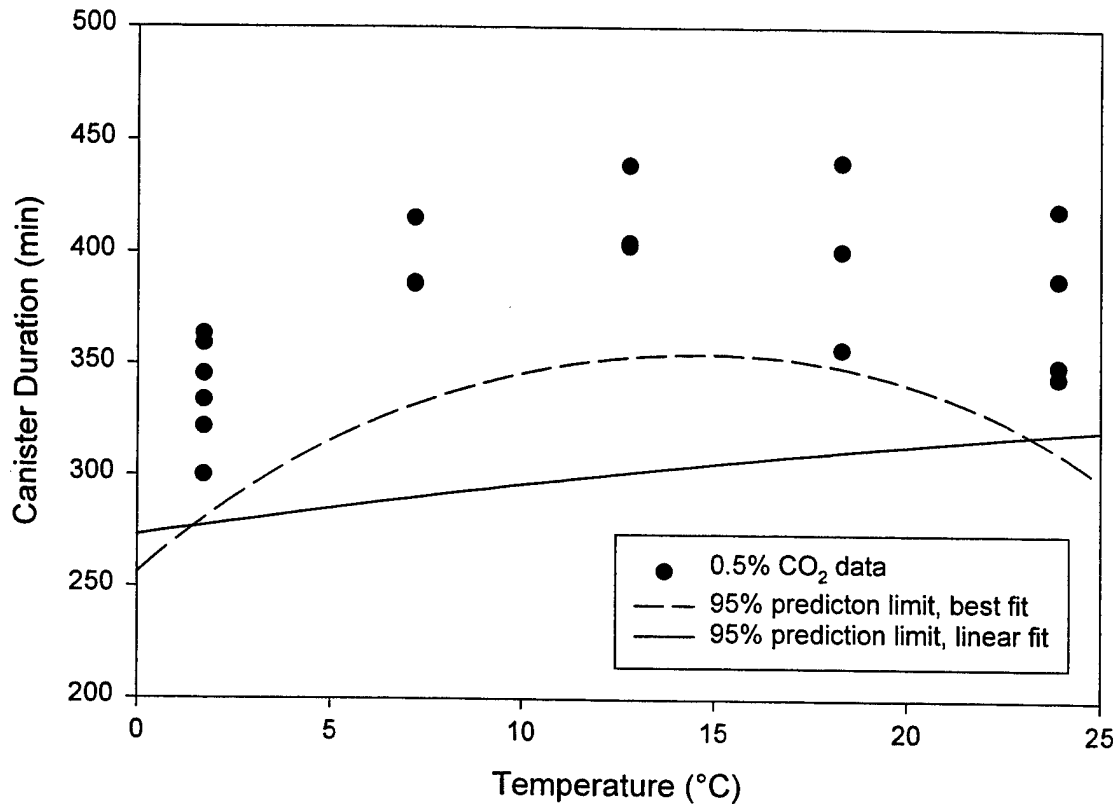
Figure 16. Comparison of the lower 95% prediction limits resulting from a linear model (solid line, F = 4.5 ) and the best fit model, a second-order polynomial (dashed line, F = 12.2 ).
