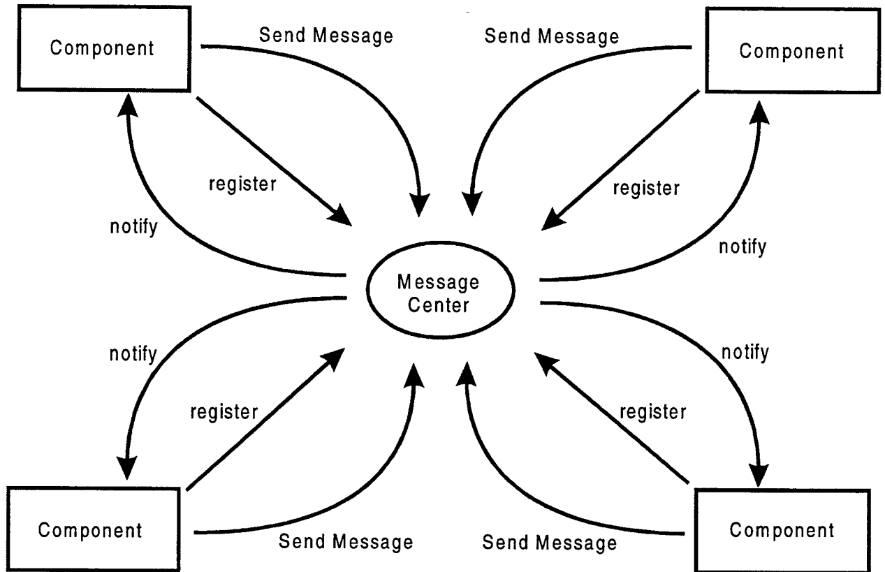
Figure 3: Software architecture.
