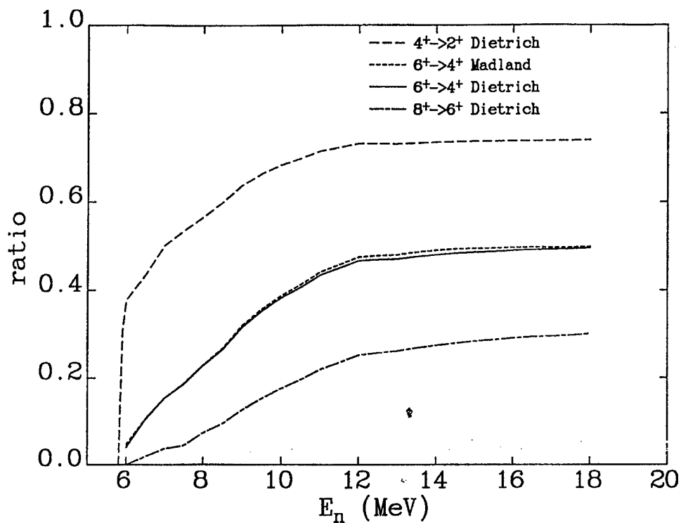
Fig 7. Ratio of ^{239}\text{Pu}(n,2n)^{238}\text{Pu}/^{239}\text{Pu}(n,2n)^{238}\text{Pu} cross section for the 8^+ , 6^+ , 4^+ states in ^{238}\text{Pu} .
