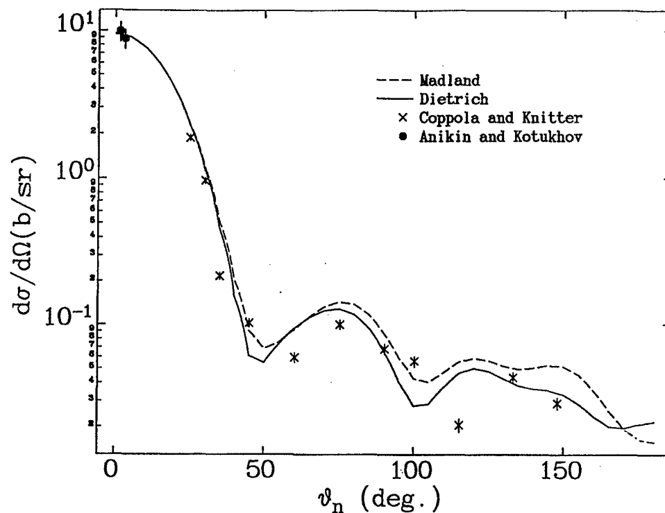
Fig. 3. Angular distribution for ^{239}\text{Pu}(n,\text{el}) at 5.5 MeV.
