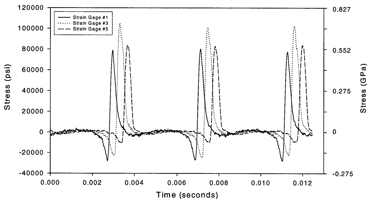
Figure 8: Dynamic data for the same conditions as Figure 7 but for three pinion revolutions.
