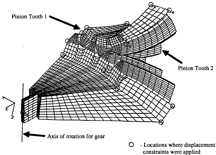
Figure 1: Seven-tooth model used in finite element analysis.
