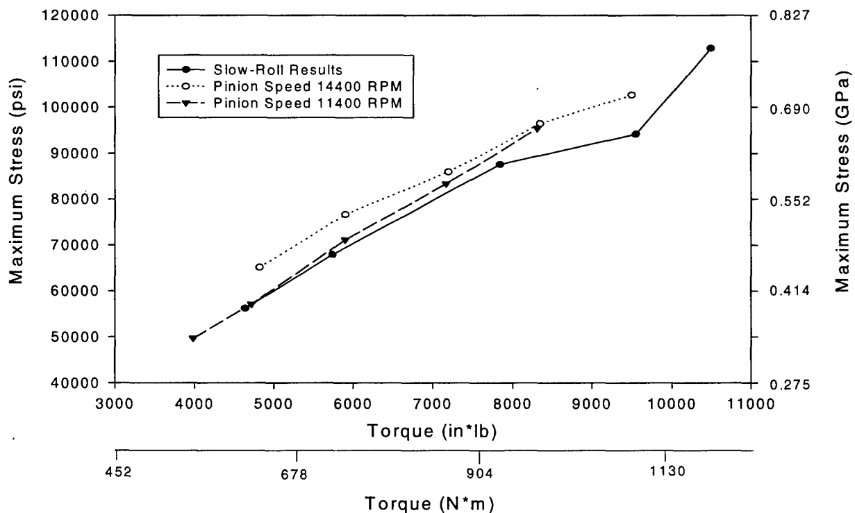
Figure 11: Comparison of slow roll data to that taken at two pinion shaft speeds. Applied torque was measured at the gear shaft.
