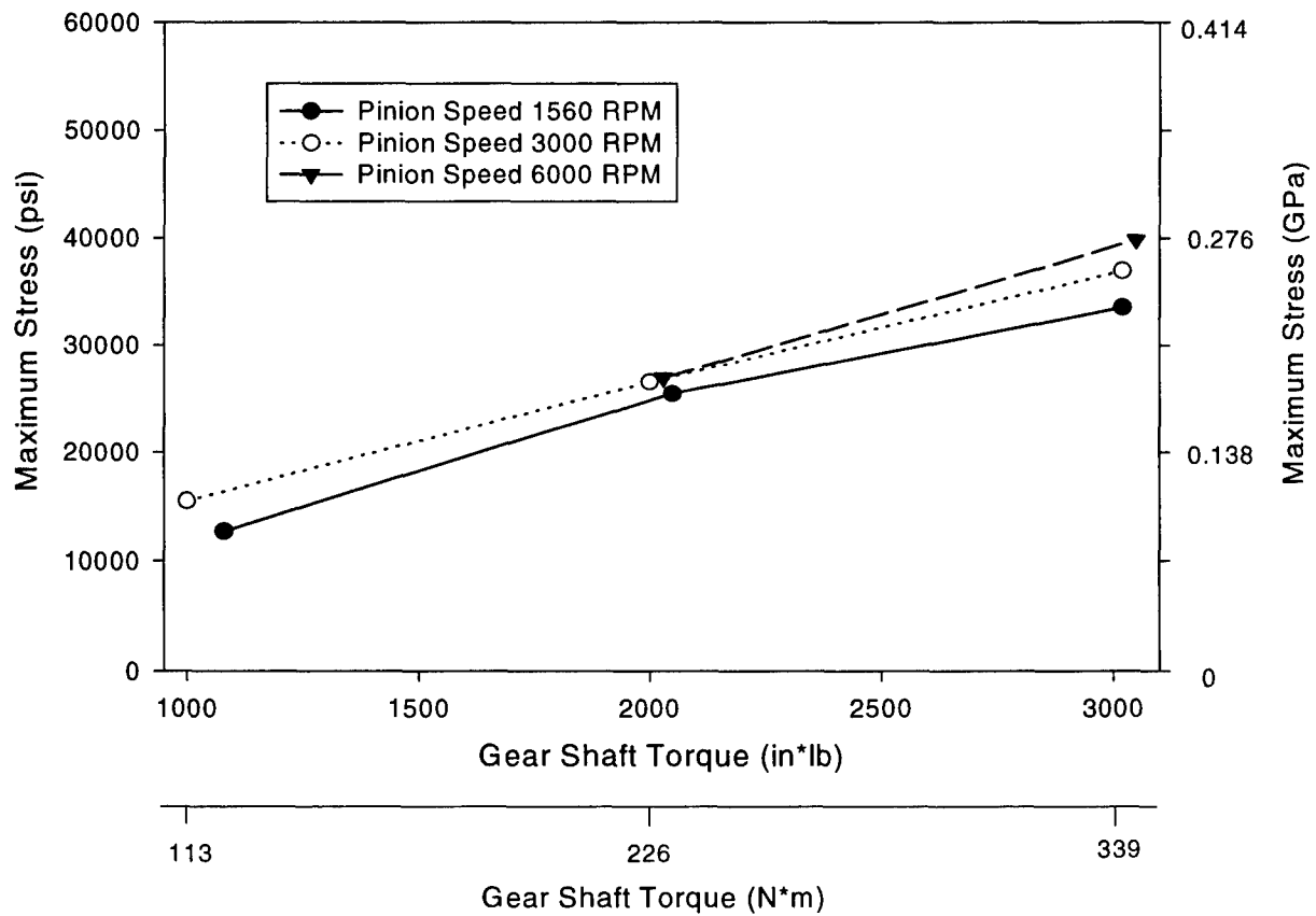
Figure 10: Effect of speed on measured maximum stress.
