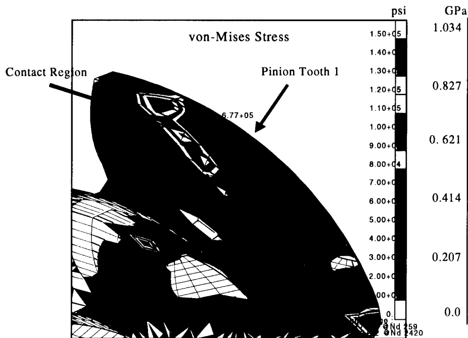
Figure 2: Example of finite element results from 3-D contact analysis at gear torque equal to 1073 N*m (9500 in*lb).
