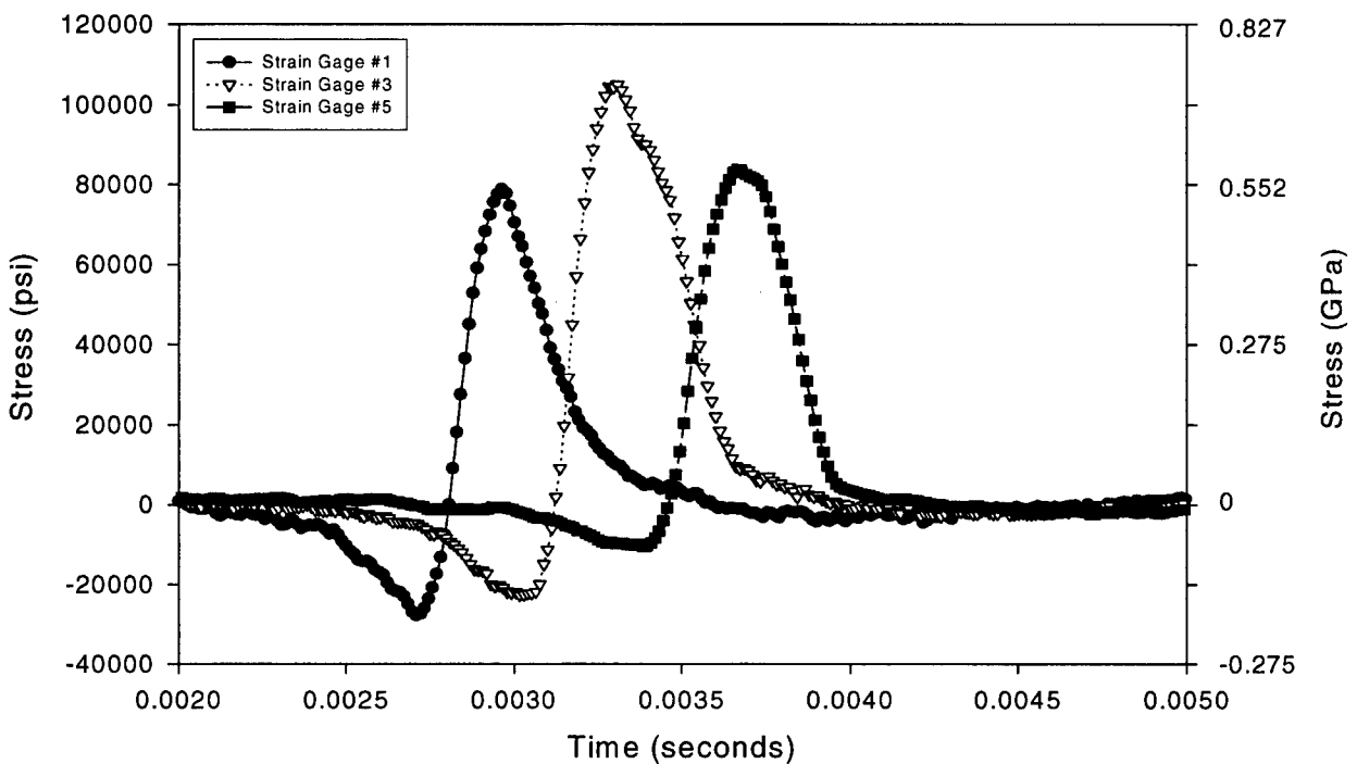
Figure 7: Dynamic data taken at pinion shaft speed of 14400 RPM, and gear shaft torque equal to 1073 N*m (9500 in*lb).
