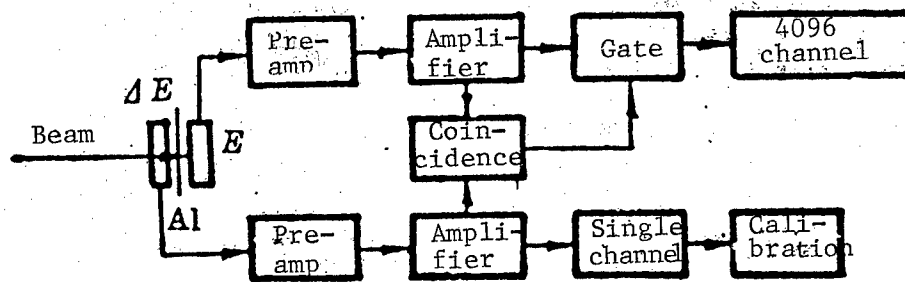
Figure 2. Measurement Circuit
