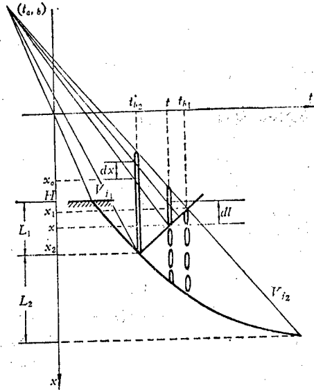
Figure 6. Penetration Calculation of Broken Jet
