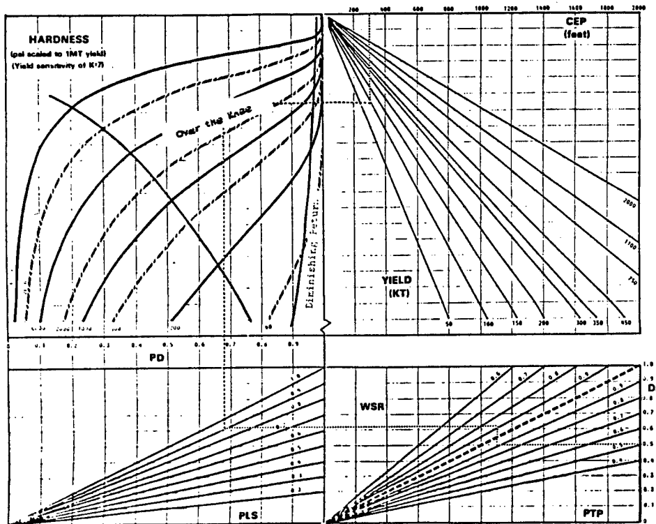
Figure 11. Hardness Regions
