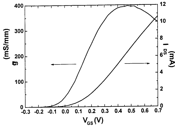
Figure 3: g_m and I_{DS} as functions of V_{GS} for a 1.0 \times 50 \text{ } \mu\text{m}^2 \text{In}_{0.25}\text{Al}_{0.75}\text{As}/\text{In}_{0.25}\text{Ga}_{0.75}\text{As} MODFET
