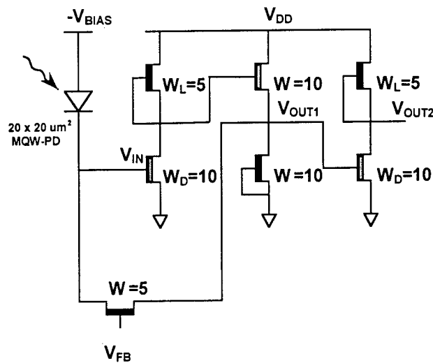
Figure 10: Transimpedance receiver circuit
