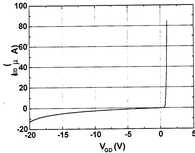
Figure 4: I_{GD} as functions of V_{GD} for a 1.0 \times 50 \text{ } \mu\text{m}^2 \text{In}_{0.25}\text{Al}_{0.75}\text{As}/\text{In}_{0.25}\text{Ga}_{0.75}\text{As} MODFET
