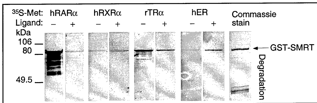
Figure 3. SMRT interacts with ER. We blotted the purified GST-C-SMRT on nitrocellulose filters and hybridized with 35 S-methionine labeled nuclear receptors in the absence or presence of hormones. We used all-trans RA for RAR, 9- cis RA for RXR, T3 for TR and 17 \beta -estradiol for ER at 1 \mu M concentration). The last lane shows the GST-SMRT fusion protein on the gel after staining by commassie blue. These results indicate that SMRT are not only capable of interacting with unliganded RAR and TR, but also capable of interacting with ER.
