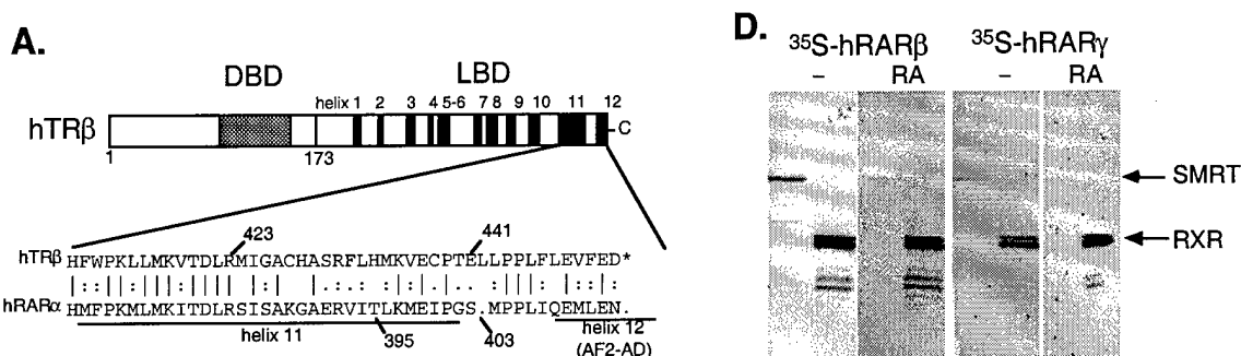
Figure 4. Two nuclear receptor domains interact with SMRT. (A) Domain structure of hTR \beta . (B) Protein-protein interactions between receptors and SMRT or RXR in far-Western analyses. (C) Summary of relative levels of interactions between receptor mutants and SMRT or RXR. (D) Human RAR \beta and RAR \gamma interact with SMRT in a ligand-reversible manner in far-Western blots.
