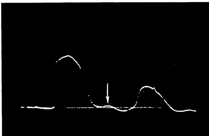
(b) Manganin gage record showing for fracture signal (arrow) arising from damage at spall plane.
