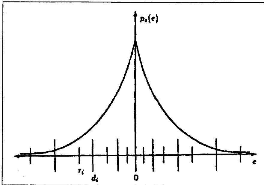
Figure 9 Typical Eight level Lloyd-Max Quantizer Distrubution
