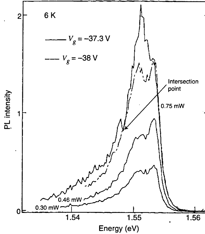
Figure 3. Observed 6 K PL spectra for I = 0.3, 0.46 , and 0.75 mW with V_g = -37.3 V (solid lines) and I = 0.75 mW, V_g = -38 V (dashed lines).
