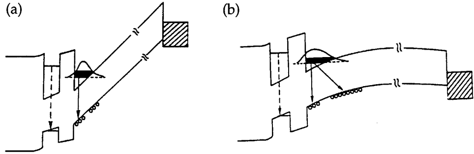
Figure 1. Schematic of backgated coupled-well bandstructure for (a) negative gate voltage and (b) positive gate voltage.
