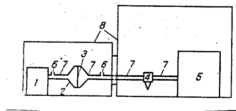
Figure 1--Model of a stand for testing the protective effectiveness of filtration materials. 1 - electro-aspirator; 2 - detachable cartridge for attachment of filtration material; 3 - filtration material; 4 - sprayer; 5 - compressor; 6 - sample collection openings; 7 - air channels; 8 - protective hermetic boxes
