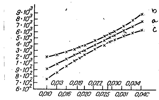
Figure 2--Regression correlation between the number of microbial bodies in 1 ml of sorbent liquid after passing through the filtration material and the filtration speed, with confidence limits of 95 percent (original concentration of bacteria in the suspension that was sprayed was 2.72 \cdot 10^6 \pm 0.37 microbial bodies in 1 ml). a - regression correlation between the number of microbial bodies in the sorbent liquid after passing through the FPP-15 fabric and the filtration speed; b, c - upper and lower 95 percent confidence limits; the y-axis represents the number of microbial bodies in 1 ml of sorbent liquid after passing through the fabric being tested; the x-axis represents the speed of the air passing through the fabric (m/sec).
