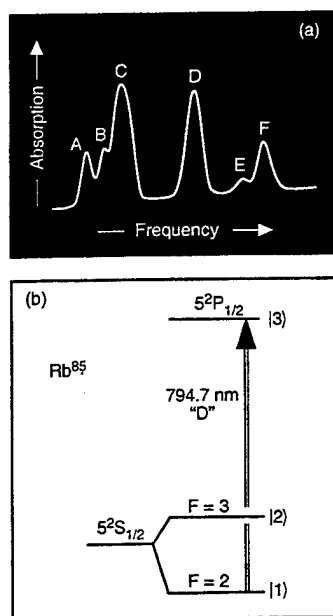
FIG. 2. (a) Absorption spectrum of the natural Rb vapor (i.e., 72% \text{Rb}^{85} and 28% \text{Rb}^{87} ) as measured with the 56-MHz linewidth diode laser at 794.7 nm and at a temperature of 32^\circ\text{C} : (A) 5^2P_{1/2}(F=1) \rightarrow 5^2S_{1/2}(F=2) transition for \text{Rb}^{87} ; (B) 5^2P_{1/2}(F=2) \rightarrow 5^2S_{1/2}(F=2) transition for \text{Rb}^{87} ; (C) 5^2P_{1/2}(F=2,3) \rightarrow 5^2S_{1/2}(F=3) transition for \text{Rb}^{85} ; (D) 5^2P_{1/2}(F=2,3) \rightarrow 5^2S_{1/2}(F=2) transition for \text{Rb}^{85} ; (E) 5^2P_{1/2}(F=1) \rightarrow 5^2S_{1/2}(F=1) transition for \text{Rb}^{87} ; (F) 5^2P_{1/2}(F=2) \rightarrow 5^2S_{1/2}(F=1) transition for \text{Rb}^{87} . The ground-state hyperfine splitting of \text{Rb}^{85} is 3036 MHz, while that of \text{Rb}^{87} is 6835 MHz. The 5^2P_{1/2} excited-state hyperfine splitting of \text{Rb}^{85} is 362 MHz, and unresolved within the Doppler-broadened absorption line, while that of \text{Rb}^{87} is 812 MHz. (b) Relevant energy-level diagram for the D transition of (a).
