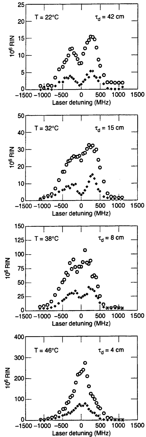
FIG. 3. RIN (multiplied by 10^6 ) vs laser detuning. Black diamonds correspond to the results obtained with the EC laser, while circles correspond to the results obtained with the TJS diode laser.
