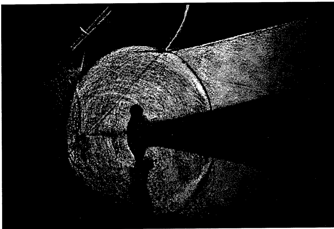
Figure 8. A schlieren image shows a spherical shock generated by the laser plasma at the target at 6 \mu\text{s} after the laser pulse. The laser energy is approximately 150 J. A conical shock can also be seen at the right side of the frame caused by rapid heating and expansion of water in the focal volume (dark conical volume).
