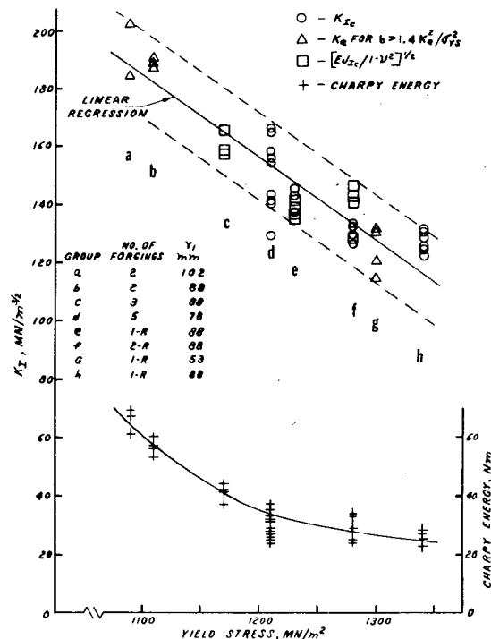
Fig. 7—Fracture toughness and Charpy energy vs. yield stress for cannon forgings
