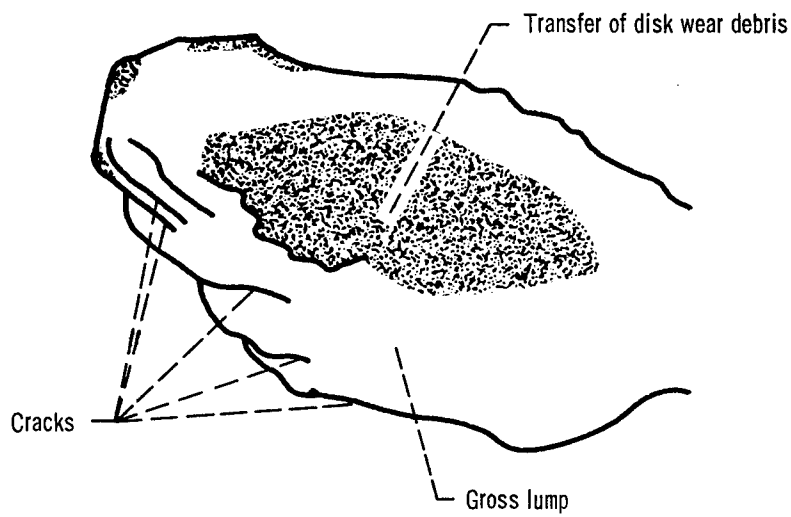
Figure 8. - Wear scar on iron-chromium alloy (14 wt. % Cr) rider showing lump and cracks.
