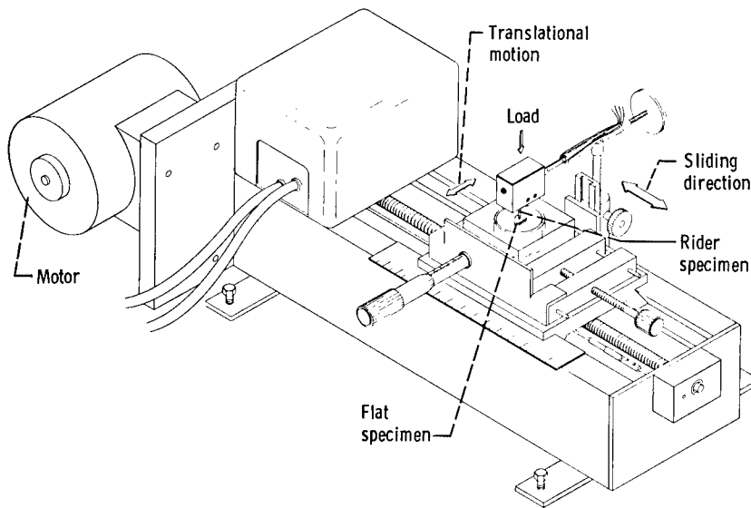
(b) Abrasive wear apparatus. Figure 1. - Friction and wear apparatus.
