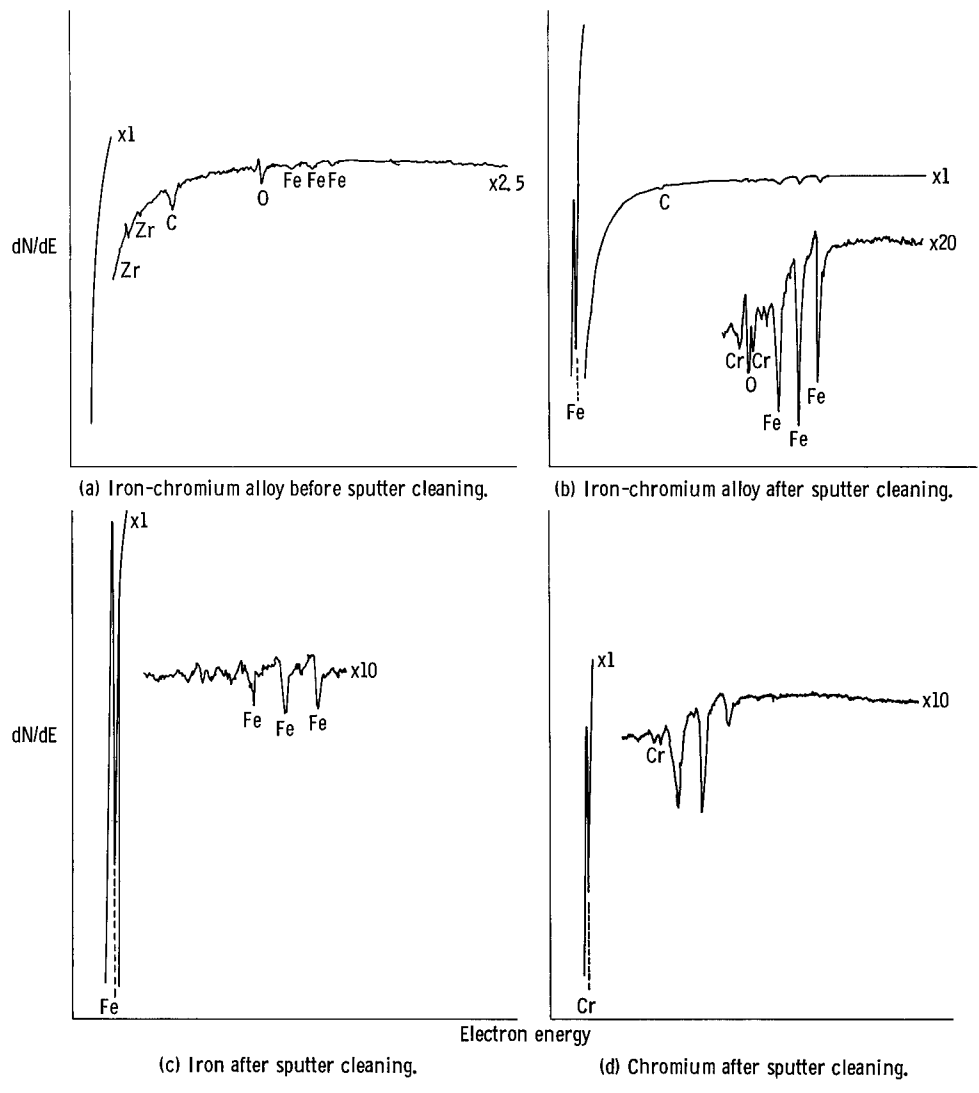
Figure 2. - Auger emission spectra for 14 weight percent iron-chromium alloy, iron, and chromium surfaces.
