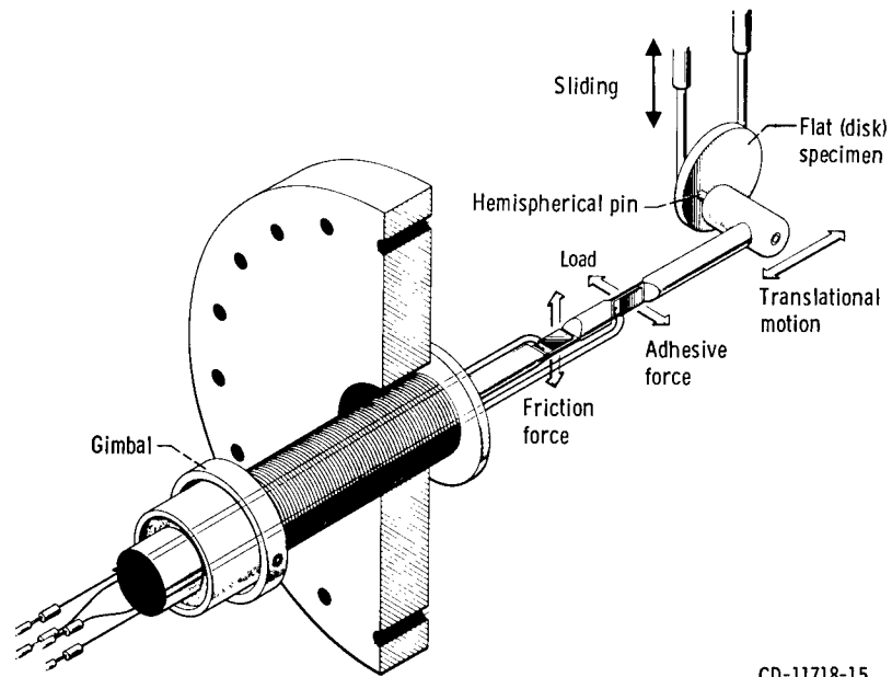
(a) Adhesive-wear apparatus.
