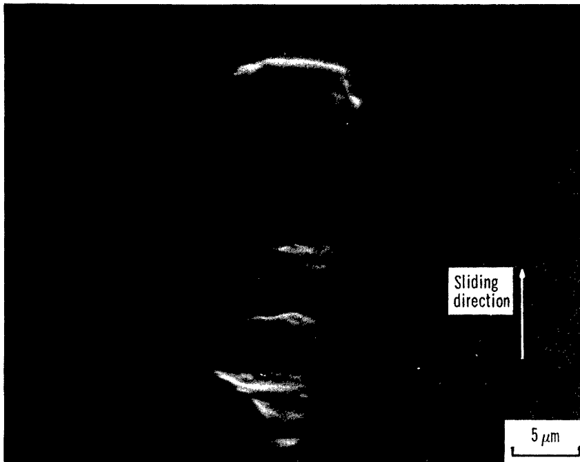
(b) Indentations on disk .
