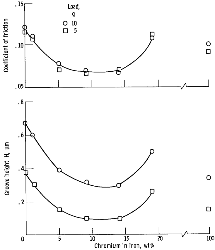
Figure 15. - Coefficient of friction and groove height for Fe-Cr alloys, iron, and chromium as result of single-pass sliding of 0.025-millimeter-radius silicon carbide rider in mineral oil. Sliding velocity, 3 mm/min; room temperature.
