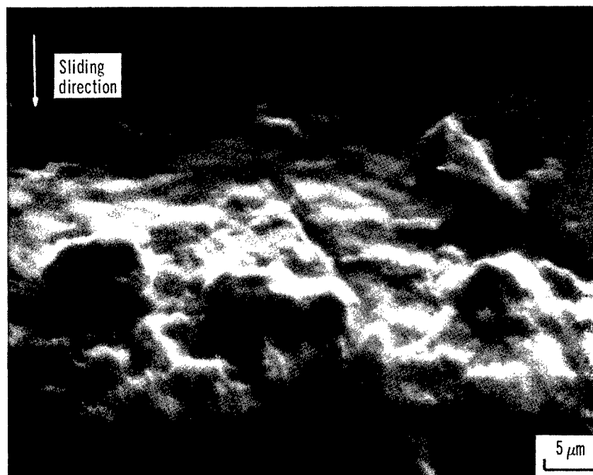
Figure 7. - Wear track on iron-chromium alloy (14 wt. % Cr) disk produced during sliding contact with itself. (Scanning electron micrographs)
