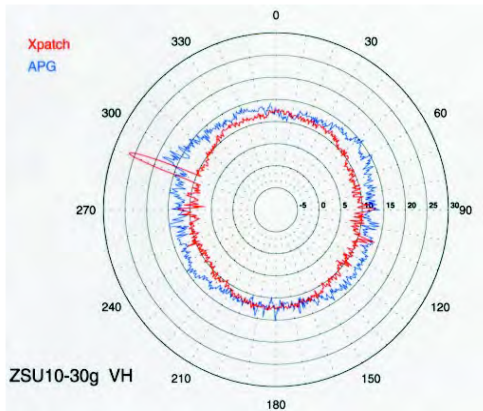
Figure 6. Comparison of Xpatch and APG RCS data for ZSU measurement at X-band, 30^\circ depression angle, cross-polarized field components (vertical transmit, horizontal receive). Xpatch results are for a vehicle with a ground plane.
