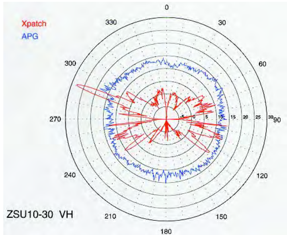
Figure 5. Comparison of Xpatch and APG RCS data for ZSU measurement at X-band, 30^\circ depression angle, cross-polarized field components (vertical transmit, horizontal receive). Xpatch results are for a vehicle without a ground plane.
