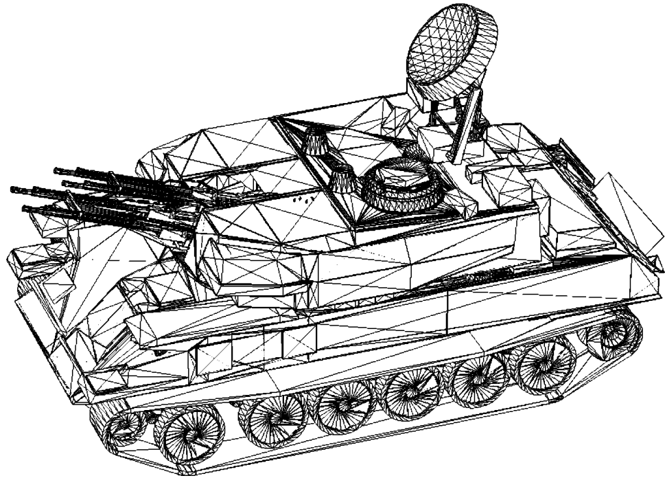
Figure 8. Facet model of the ZSU at 30° depression angle and 290° in azimuth angle.
