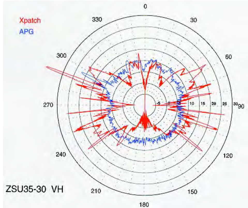
Figure 7. Comparison of Xpatch and APG RCS data for ZSU measurement at K_a -band, 30^\circ depression angle, cross-polarized field components (vertical transmit, horizontal receive). Xpatch results are for a vehicle without a ground plane.
