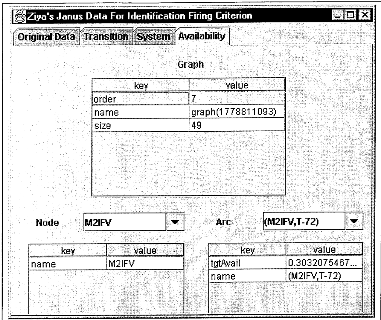
Figure 13. Another sample output of the JAVA program that displays final target availability information for all M2IFVs of all T-72 tanks. The menu item "Transition" on top of the figure displays the menu where the transition rates were calculated for each entity. The menu item "System" displays the information on total systems transition rates for weapon types such as M1A1 tanks. The menu item Original Data is displayed in Figure 12.
