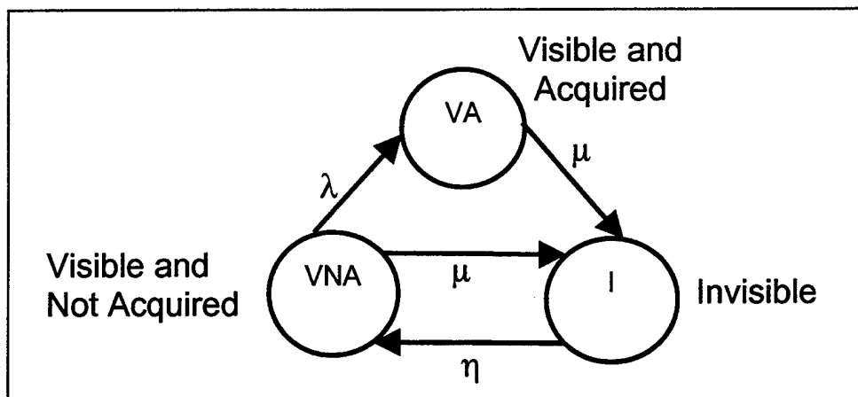
Figure 8. The original three-state Markov chain model of non-firing target acquisition suggested by Gordon Clark.
