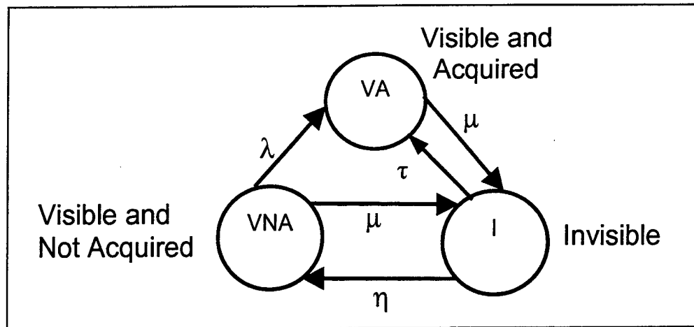
Figure 9. The modified version of the original three-state Markov chain model of non-firing target acquisition suggested by Gordon Clark. During the research effort, the author of this thesis discovered that JANUS allows a transition from the Invisible state to the Visible and Acquired state.
