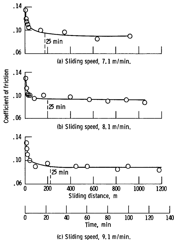
Figure 5. - Coefficient of friction as function of sliding distance and time for C-ether-base lubricant. Load, 1 kilogram; disk speed, 50 rpm; atmosphere, dry air; disk temperature, 20° C; pure iron rider on M-50 disk.
