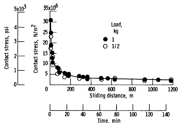
Figure 6. - Contact stress as function of sliding distance and time for ester-base lubricant. Disk speed, 50 rpm; atmosphere, dry air; disk temperature, 20° C; pure iron rider on M-50 disk.
