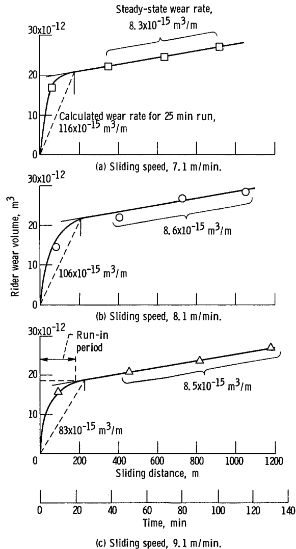
Figure 4. - Rider wear as function of sliding distance and time for C-ester-base lubricant. Load, 1 kilogram; disk speed, 50 rpm; atmosphere, dry air; disk temperature, 20° C; pure iron rider on M-50 disk.
