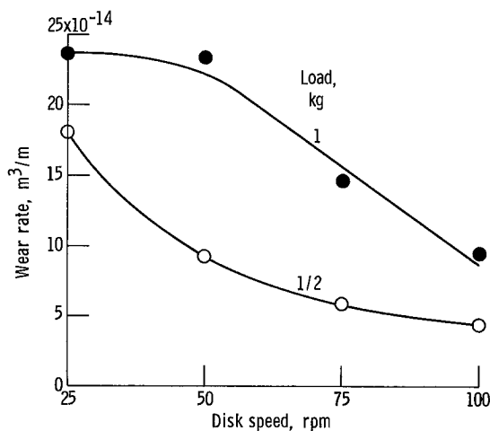
Figure 3. - Effect of disk speed on rider wear rate at two loads with ester-base lubricant. Atmosphere, dry air; disk temperature, 20° C; pure iron rider on M-50 disk.
