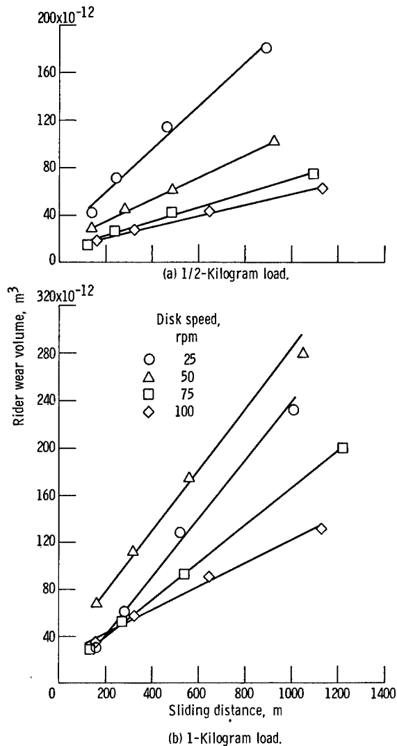
Figure 2. - Rider wear as function of sliding distance for an ester-base lubricant. Atmosphere, dry air; disk temperature, 20° C.
