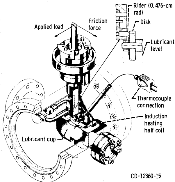
Figure 1. - Friction and wear apparatus.
