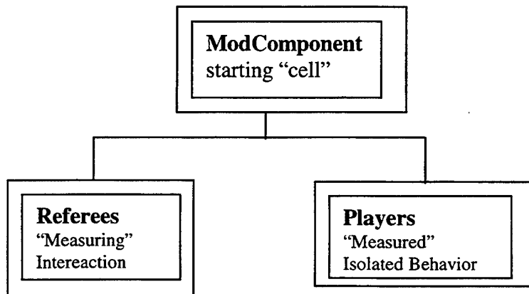
Figure 1. ModComponent Evolution
