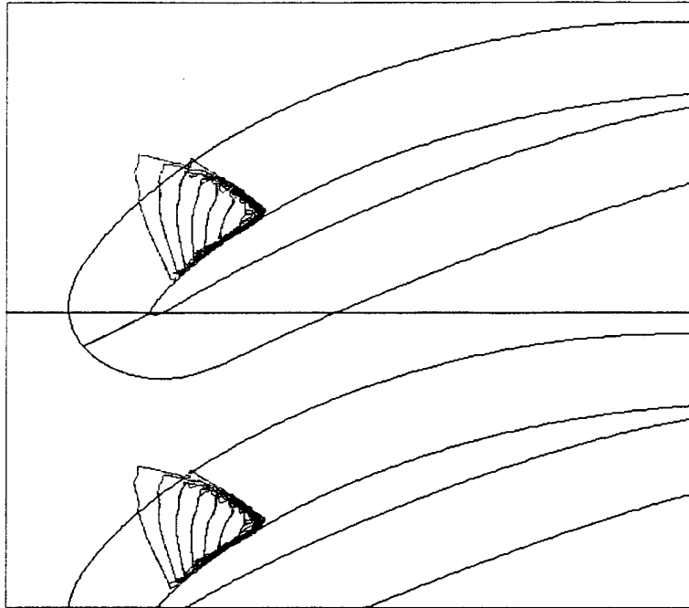
Figure 14: Mach number contours indicating extent of supersonic region in Run 4. Contours range from M = 1.0 to M = 1.5 in steps of 0.05. M_\infty = 0.87 .
