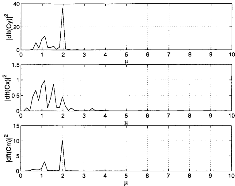
Figure 25: Discrete fourier transform of the baseline force and moment coefficients. dft(X) is the discrete fourier transform of the time signal X . \mu = \text{non-dimensional frequency} . M_\infty = 0.87 .
