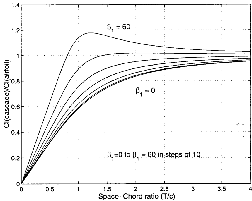
Figure 31: Cascade model results for the change in cascade interference coefficient Cl_{cascade}/Cl_{airfoil} with space-chord ratio and stagger angle. No. of panels = 5.
