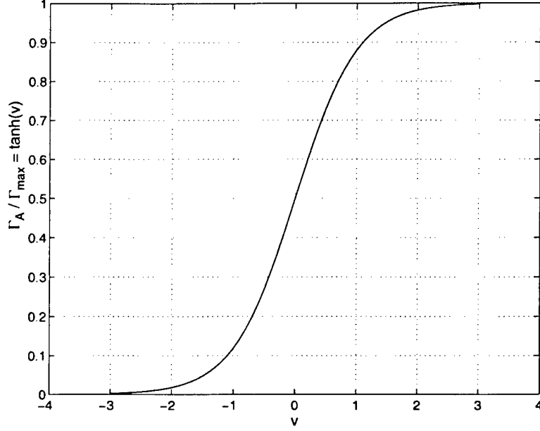
Figure 28: Change in circulation strength of the convecting vortices. v = s_1\xi + s_2 where \xi is the location of the convecting vortex and s_1 and s_2 are constants which ensure the \tanh function is evaluated between -3 and +3 .
