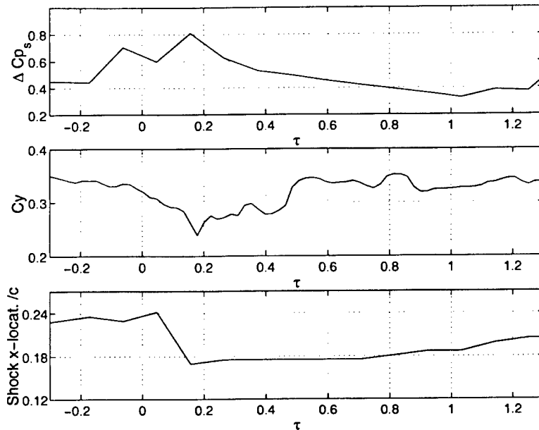
Figure 16: The change in (1) static pressure difference across the shock wave, (2) azimuthal force coefficient and (3) blade shock location during passage of a density wake width 0.1c and density ratio 0.25 . M_\infty = 0.87 .
