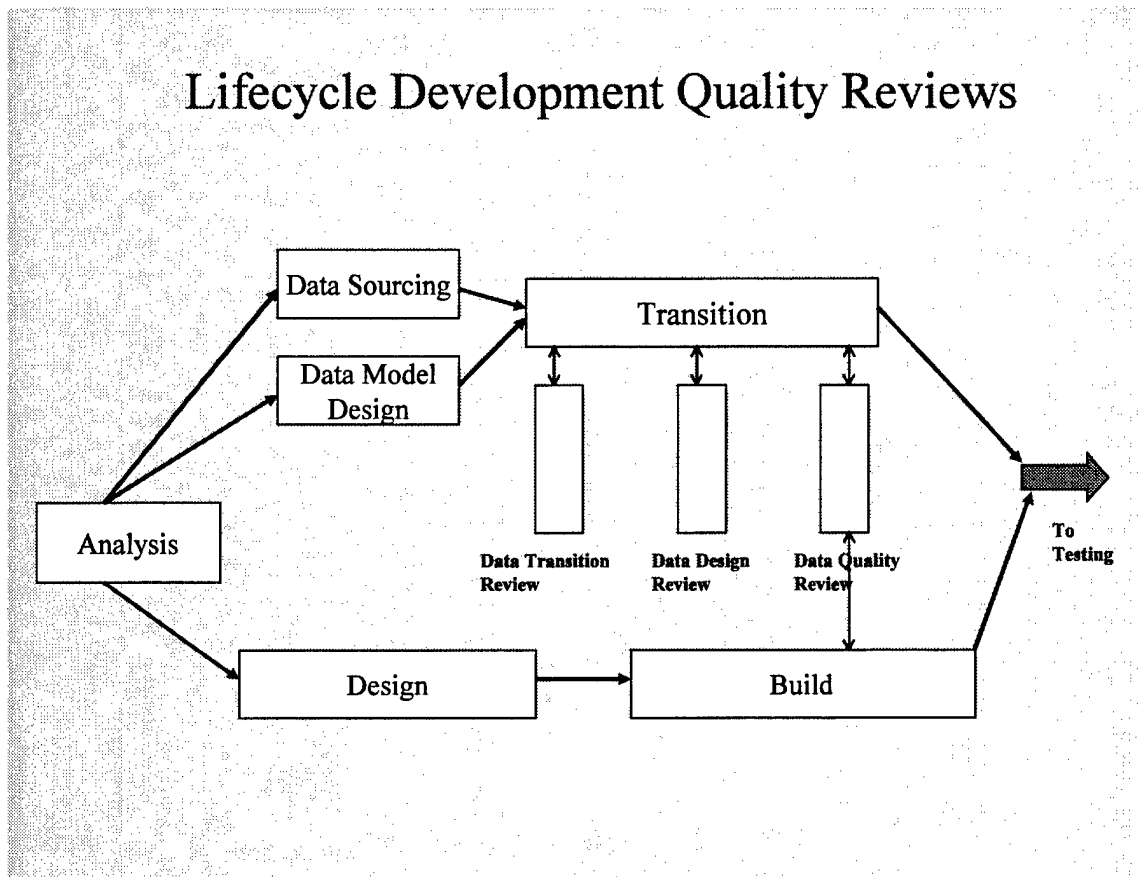
FIGURE 4-3. LIFECYCLE DEVELOPMENT QUALITY REVIEWS
