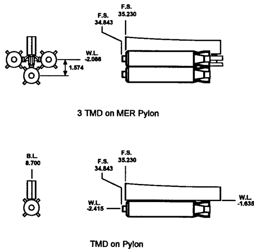
Figure 3. TMD Pylon Configurations [Ref. 4]
