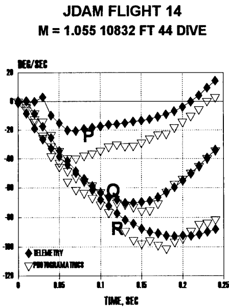
FIGURE 16 JDAM RATES
