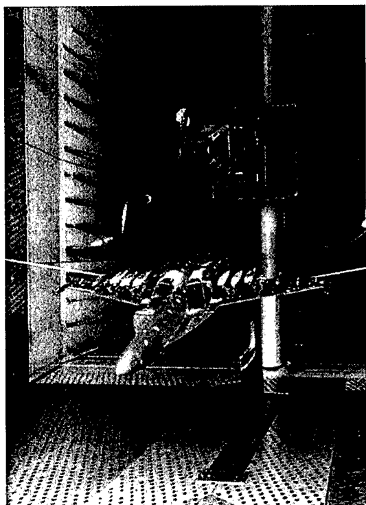
Fig 6 F/A-18E/F Model In The AEDC 16T Transonic Wind Tunnel
