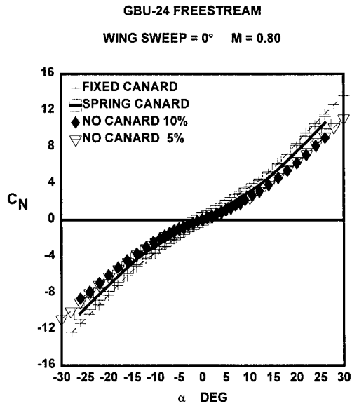
FIGURE 6: GBU-24 FREESTREAM
