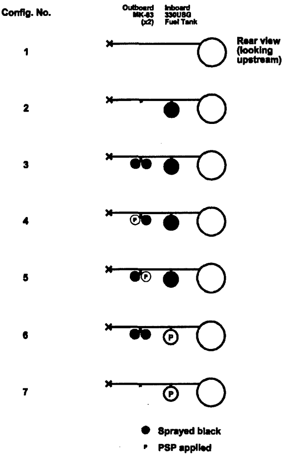
Figure 4: Stores Configurations with PSP and Sprayed Black
