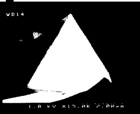
This new concept in nanolithography is based upon the transport of a chemically reactive material or "ink" from the tip of a conventional silicon nitride Atomic Force Microscope (AFM) to the surface of interest or "paper."
