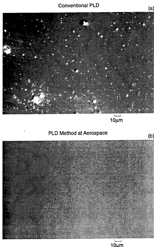
Figure 1. Surface morphology of a TiC film deposited on a 52100 steel substrate as seen in scanning electron microscopy: (a) using conventional Pulsed Laser Deposition (PLD) and (b) using the modified PLD process developed in this IR&D program.
