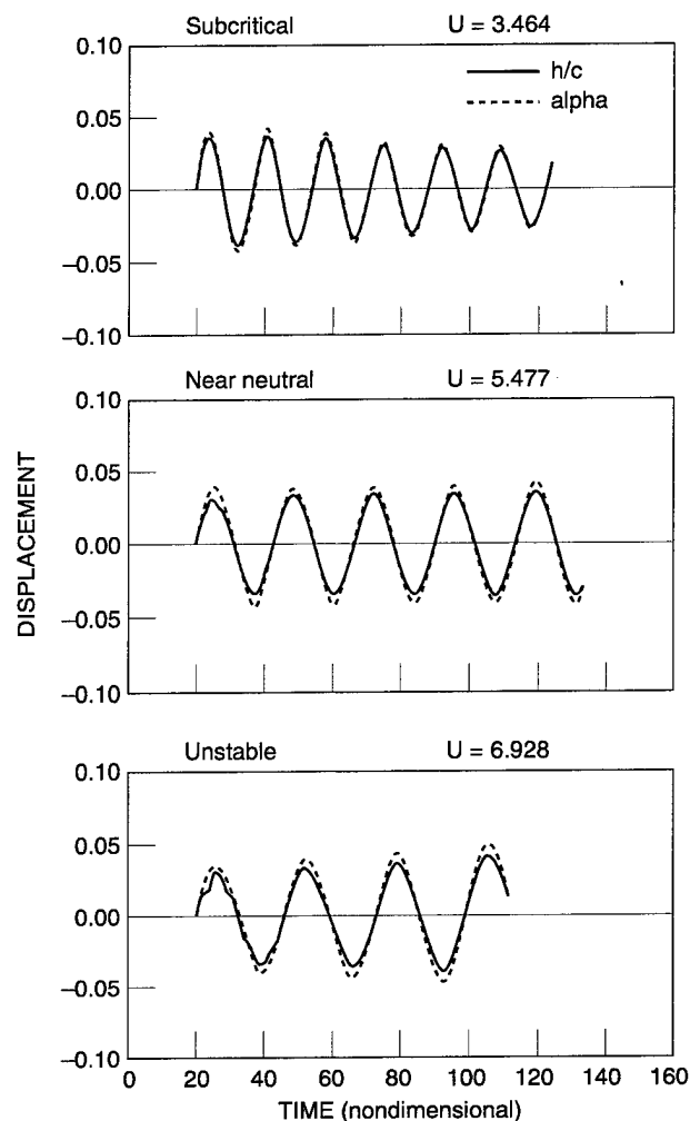
Figure 1. Transient Flutter Analysis of NACA 0012 Airfoil at M_\infty = 0.80 , \alpha_0 = 0.0 deg.
