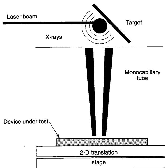
Figure 1. Collecting and focusing X-rays using a monacapillary tube.
