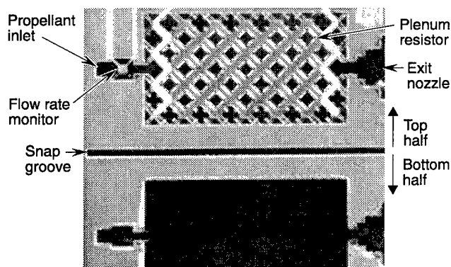
Figure 5. Photograph of part of the resistojet die after etching. The plenum resistor is a patterned polysilicon sheet sandwiched between two patterned glass layers. The plenum is 1.2 mm long and the heating element is less than 1 micron thick.
