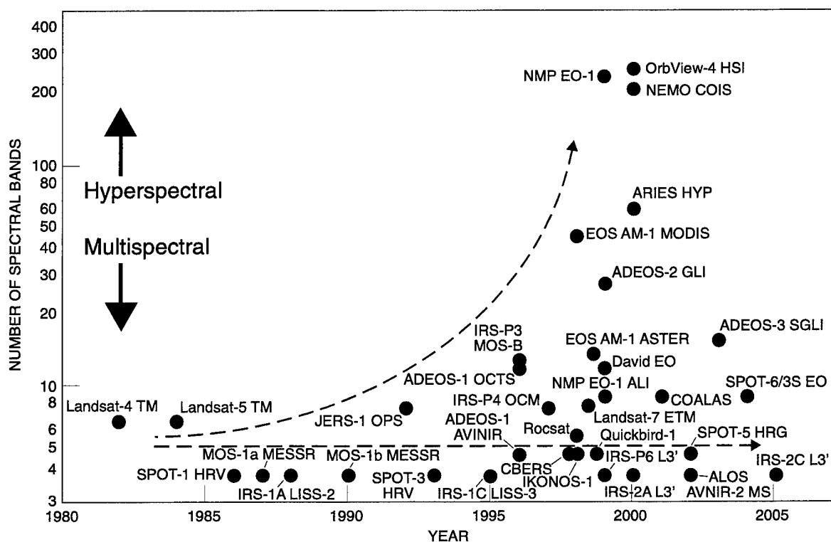
Figure 3. Diverging trends in spectral bands for civil spaceborne visible/IR imaging instruments 1980–2007.
