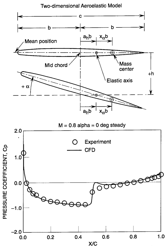
Figure 1. Transient Flutter Analysis of NACA 0012 Airfoil at M_\infty = 0.80 , \alpha_0 = 0.0 deg.
