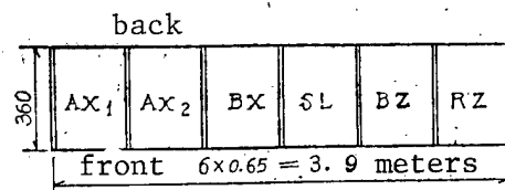
Figure 1. 200-Line Arrangement
