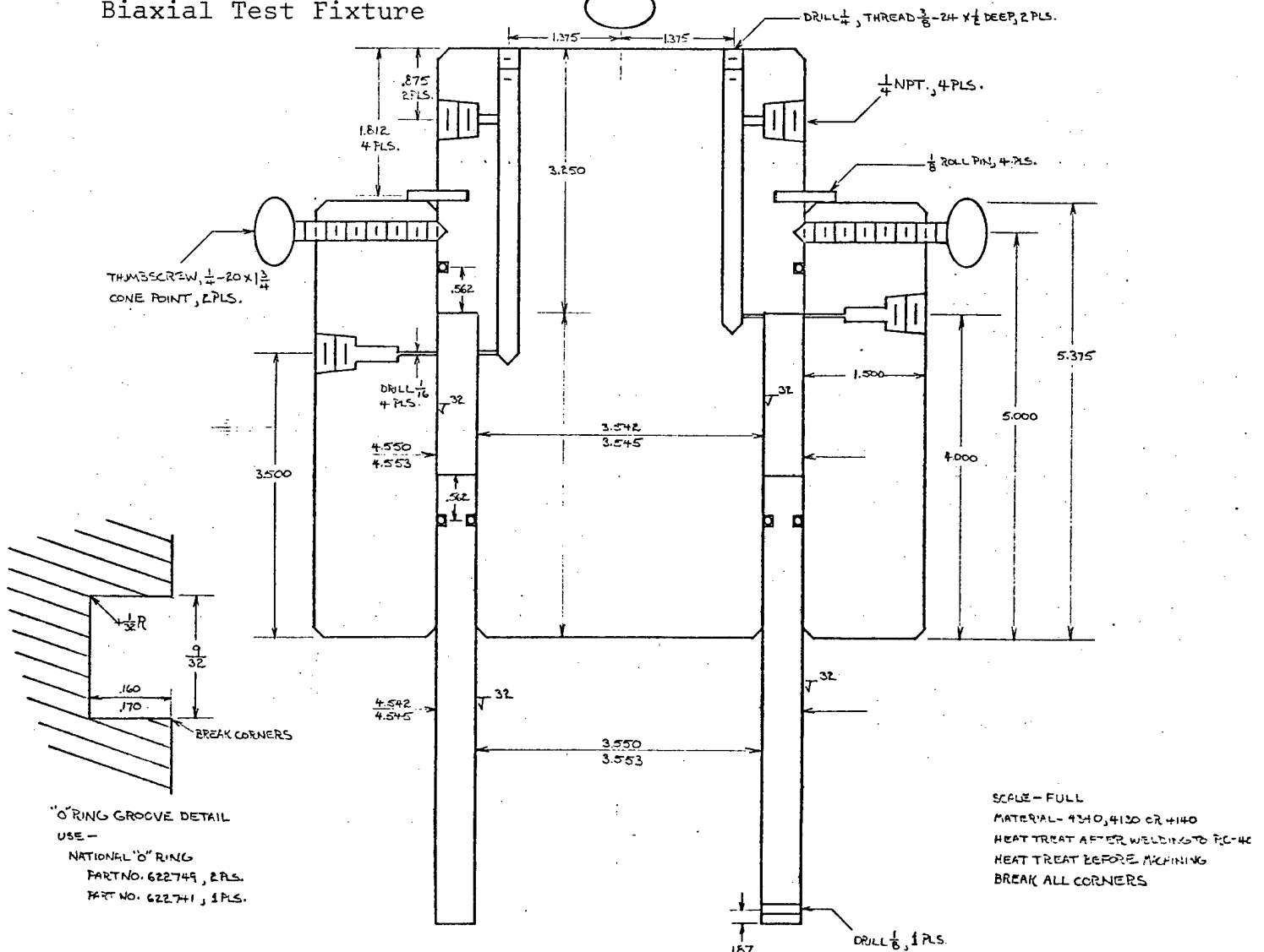
Dimensioned Drawing of Biaxial Test Fixture
